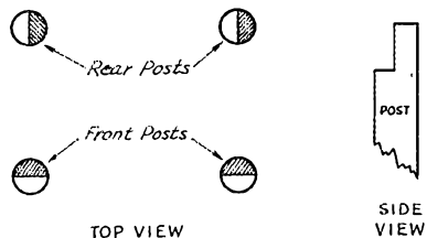
Fig. 1 — Method of anchoring legs of lattice tower to prevent strain. Shaded areas in top view indicate projecting portions of stubs.
