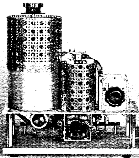
Fig. 6—The 2 1/2-meter transmitter. From left to right, the oscillator stage with the frequency control knob projecting up through the perforated shield, the W.E. 304A amplifier tube, and the amplifier tuning condenser.
