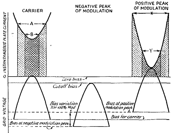
Fig. 1.—Graphical representation of the operating conditions discussed in the text. The dimension A shows the interval during which plate current flows with the conventional operating conditions, B the smaller interval with high plate voltage and high bias, both for the steady carrier. The plate loss is larger the larger the area under the curve. A similar comparison is given for the positive modulation peak, where X represents the interval of plate current flow for ordinary operating conditions and Y the corresponding interval with the method described.
