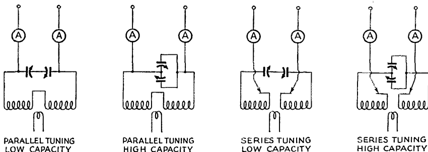
Fig. 2 — Choice of capacity range, inductance value, and series or parallel tuning is allowed by this antenna coupler. With condenser sections series-connected, a minimum capacity value of 16 to 22 \mu\text{fd.} is available, while the maximum capacity value with sections in parallel is approximately 480 \mu\text{fd.}
