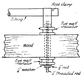
Fig. 2 — Substitute for stand-off insulators in mounting rotatable antenna elements which provides greater mechanical strength.
