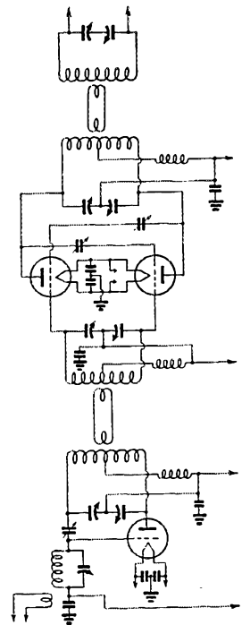
Fig. 1 — General circuit of the transmitter. Coil taps are not shown in this diagram. Aside from the high voltage connections to the tuning condenser rotors, the circuits are completely conventional. Link coupled buffer, link coupled push-pull amplifier, and link coupled antenna tuner are used for ease of obtaining correct match and loading throughout.
