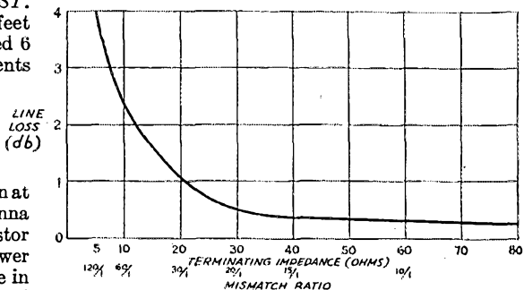
Fig. 1 -- An experimentally-determined curve of the line loss in a 1½ wavelength long 600-ohm line with various degrees of mismatch.
