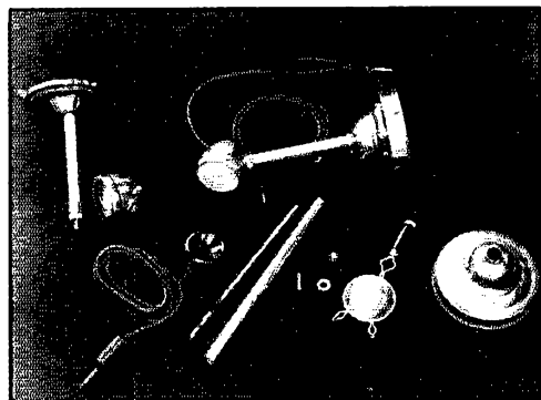
Crystal microphone made from crystal headphone unit and odd parts. The electric fixture canopy in the lower right is the base, the tea strainer forms the wire grille. A piece of nicked pipe is used for the standard and the shell of an automobile cowl light makes a good-looking head.
