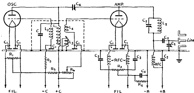
Fig. 5—The schematic wiring diagram of the 5- and 2 1/2-meter transmitters shown with the output arranged for connection to a coaxial line. The dotted line encloses the schematic representation of the oscillator tank circuit. By-pass condensers that were formed by metal strips separated from the grounded metal chassis by mica sheets are represented by a short line directly above and parallel to the ground plane. The amplifier "C" supply also furnishes plate power for the oscillator. Hence the oscillator filament is not grounded for d.c.
