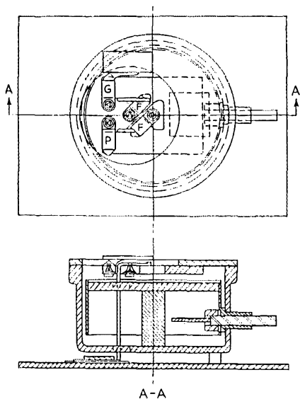
Fig. 4—A simplified assembly drawing of the Hartley type of 1 1/4-meter tank circuit. The W.E. 316A isolantite socket is shown with the filament connections passing through the field of the inductance and with the grid terminal by-passed to the top cover-plate. A cylindrical aluminum shield, which is not shown, is used to complete the shielding around the tube.
