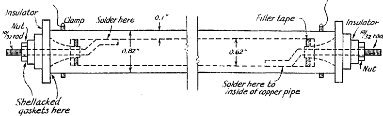
Fig. 2 — The coaxial line from the pick-up coil to the antenna is made of thin-wall electrical conduit with a piece of 1/32-inch copper tubing running through the center. Parts of feed-through insulators support the inner conductor, and the line is made weatherproof by sealing at both ends.
