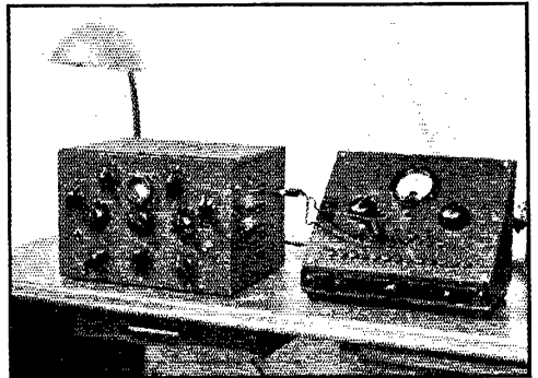
Fig. 2 — The set-up used in making the measurements. The oscilloscope on the left is connected to the d.c. voltmeter at the right by two flexible leads. Reading from left to right on the voltmeter, the controls are: range switch, r.m.s. toggle switch, and the potentiometer which controls the d.c. output.
