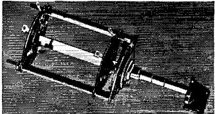
This Mallory-Yaxley Hamswitch No. 151L permits the use of a single meter to measure currents or voltages on up to and including five circuits in an amateur transmitter.
