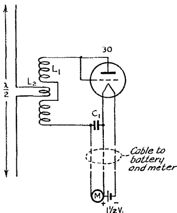
Fig. 1 — Wiring diagram of the simple field-strength indicator.
