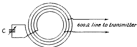
Fig. 1—The 600-ohm line from the transmitter is tapped on to one turn of a 4-turn tank coil which is tuned by condenser C. A one-turn pick-up coil is inductively coupled to the four-turn coil and feeds the antenna through a short section of coaxial line.
