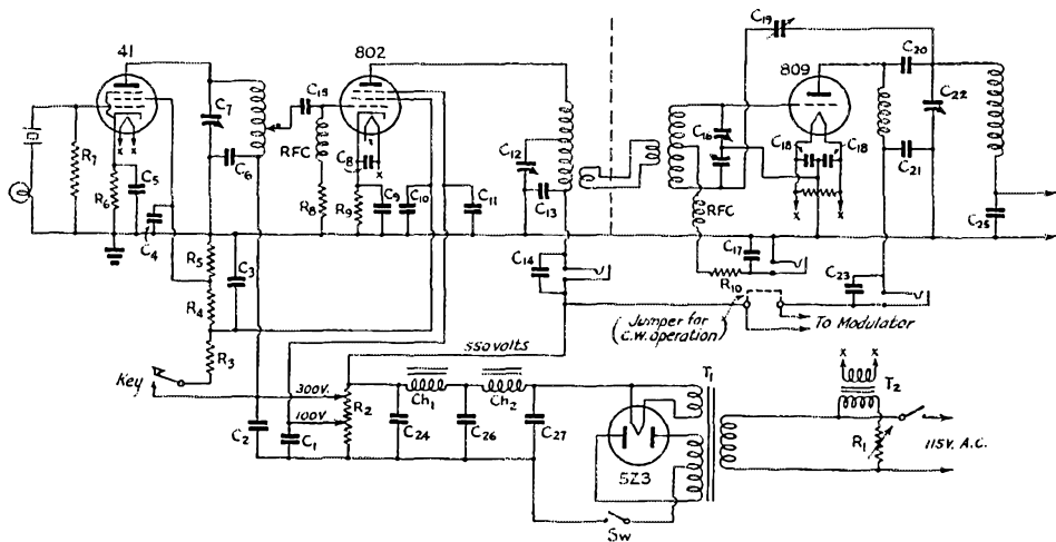
Fig. 2—Wiring of the transmitter when used for 'phone.
