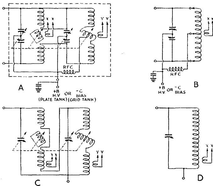
Fig. 1—Actual connections of the 5-band tank circuits (A and C) with their corresponding simplified equivalents at the right (B and D). A and B are balanced circuits for push-pull or plate neutralized amplifiers, C and D single-ended circuits.
