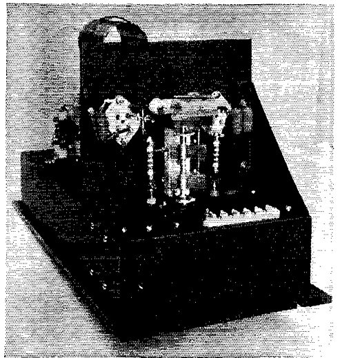
The grid end of the amplifier. The filament by-pass condensers, grid blocking condensers and r.f. chokes are arranged symmetrically about the tank coil and condenser.
