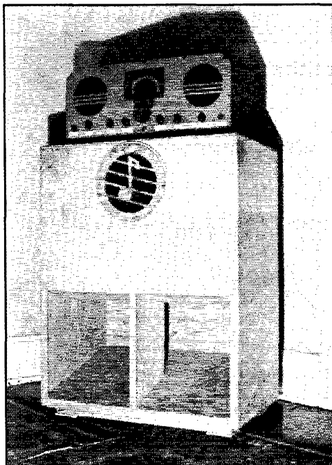
A simple homemade exponential horn with an ACR-155 mounted on top to give an idea of the size of the gadget. The low notes pass through the horn and come out at the bottom — the high notes are radiated directly through the grille at the top.
