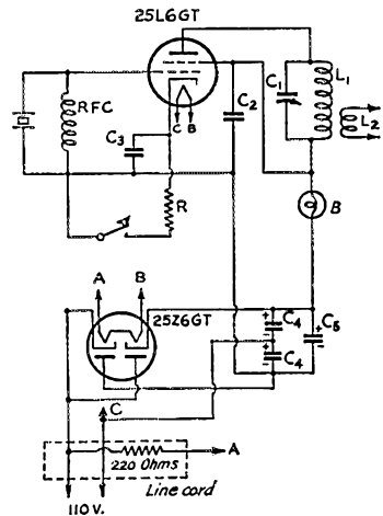
Fig 1—The "Portable Five" Circuit Diagram.
