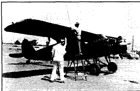
Gilbert de la Laing, W6BJI, mounts two half-waves in phase on the wing of the Stinson monoplane used in setting the 255-mile record for 112 Mc. on July 4th. Pilots Joe Bailey and Denny Whitney look on.
