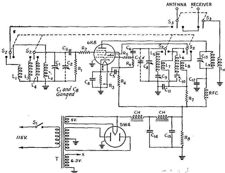
Fig. 1 — Circuit Diagram of the Low-Frequency Converter.
