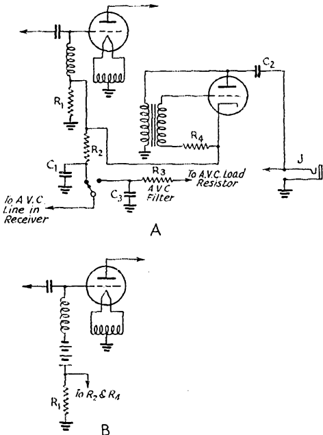
Fig. 2 — Break-in keying-monitor system with automatic receiver blocking. R_1 is the usual grid-leak resistance recommended for the stage in use. R_2 is a 0.1 meg. 1-watt resistor. A capacity of 0.25 \mu\text{fd.} is recommended for C_2 , although this capacity may be varied for a change in delay. C_3 is 0.01 \mu\text{fd.} C_3 and R_3 form the usual a.v.c. filter in the receiver.
