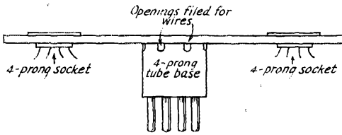
Fig. 1 — Adapter for replacing type 83 rectifier with type 866 jr.'s for higher voltages. If the rectifier filament transformer has no center tap, make positive high-voltage connection at center of series-connected filaments. The strip is fastened to the tube base by a 6-32 screw running through the center of the tube base.
