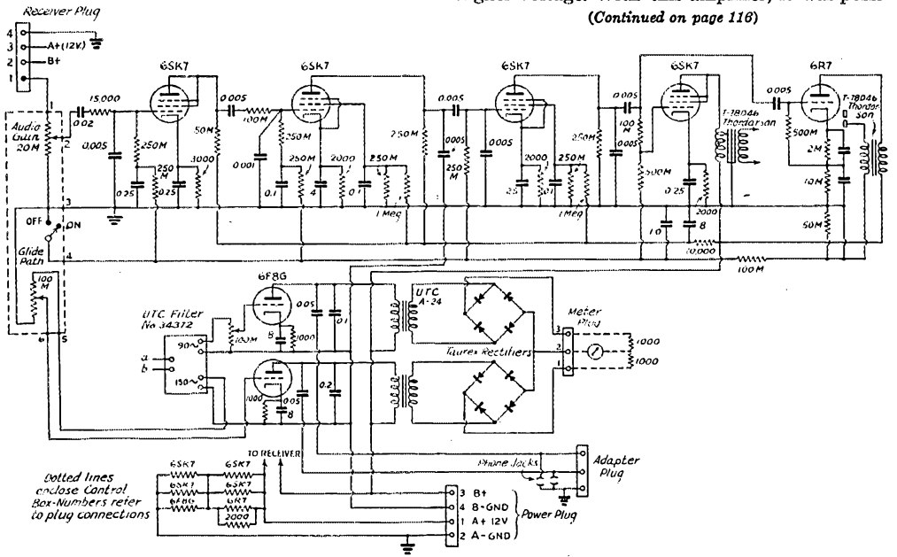
Fig. 8 — The audio amplifier-filter circuit.
