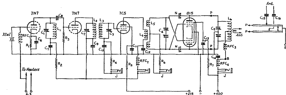
Fig. 1 — Circuit diagram of the 815 u.h.f. transmitter.
