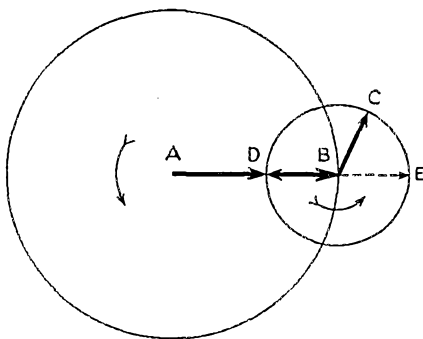
Fig. 1—Ordinary amplitude modulation, showing the effect of noise superimposed on the incoming carrier.
