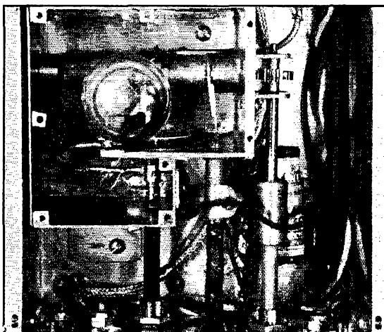
Fig. 4 — The r.f. layout is shown in this view. The special diode is in a knob-shaped bulb, mounted over the inner conductor of the concentric-line tuner. The tuned circuit through which the oscillator output is introduced is just below it. Input tuning is accomplished by means of the rack and pinion at the right, which drives the movable section of the line back and forth.
