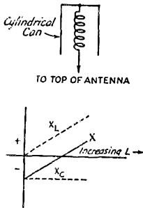
Fig. 3—Method of inserting reactance at the top of the antenna, with curve showing net reactance variation as the value of L is increased, the top capacity being fixed. For a cylinder with diameter equal to length, the capacity in \mu\text{mf.} is 2.04 times the diameter in inches.
