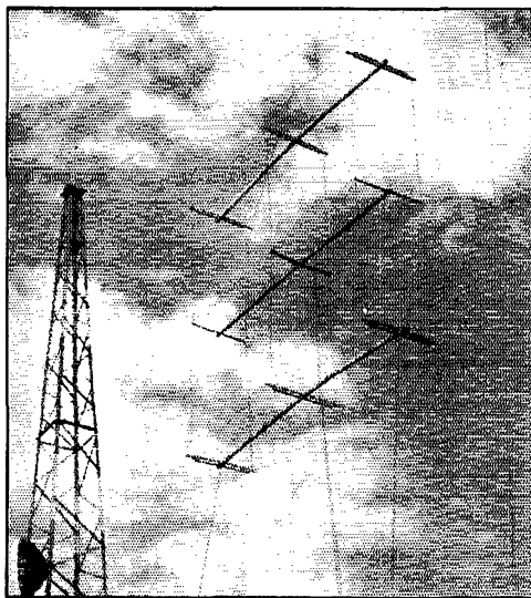
Suspended 110 feet above ground, from a 75-meter flat-top on the roof of the Institute of Geographical Exploration at Harvard University, this 12-element rotary array is largely responsible for the excellent coverage enjoyed by frequency-modulated W1ELP.
