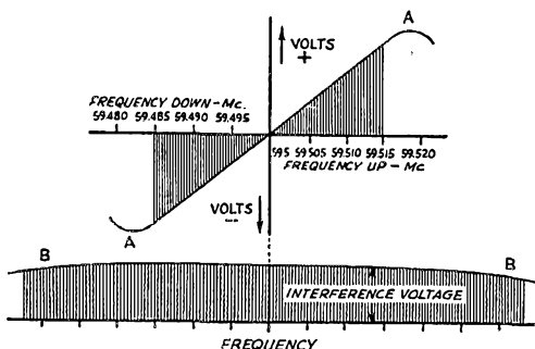
Fig. 3—Illustrating discriminator operation on frequency-modulated signals and on noise which is equally distributed in frequency and amplitude over the pass-band of the receiver.
