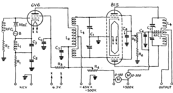
L 1 — 21 turns No. 24 d.s.c., close-wound, \frac{1}{2} -inch diam. (See Fig. 2 for specifications of L 2 and L 3 .)
