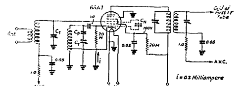
Fig. 7 — The 6SA7 converter circuit.
