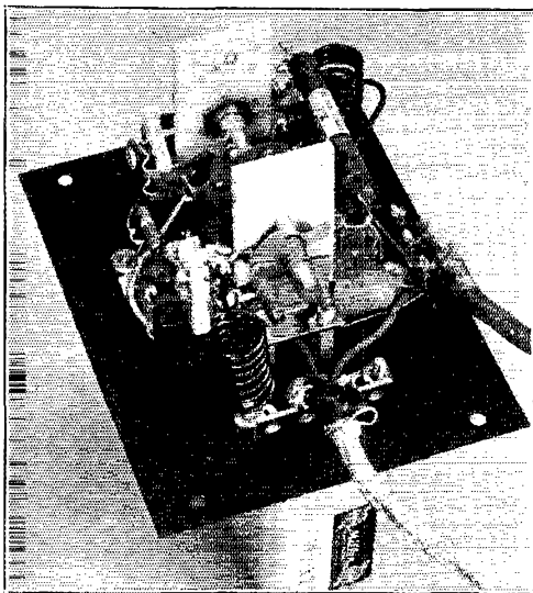
This view shows the mixer tuning condenser in the foreground. The paper by-pass condenser, C_{10} , can be seen under the right-hand side of the tuning condenser, and the screen dropping resistor, R_3 , runs under it.
