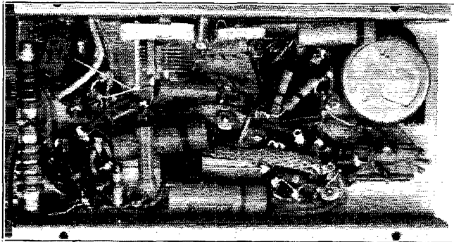
In this below-chassis view, the socket for the 6SQ7 is in the upper left corner, with the first limiter socket just below it. The two series chokes forming the shunt inductance in the i.f. circuit are along the left edge. Wiring is crowded, but i.f. leads are kept as short as possible. Rubber-covered pair runs out the lower left corner to the filament transformer.
