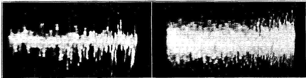
Fig. 3 — Oscillograms of internal receiver noise appearing at the frequency modulation receiver output. A (left) is with carrier-to-noise ratio at the threshold or "sputter point." B is with carrier-to-noise ratio above the threshold.
