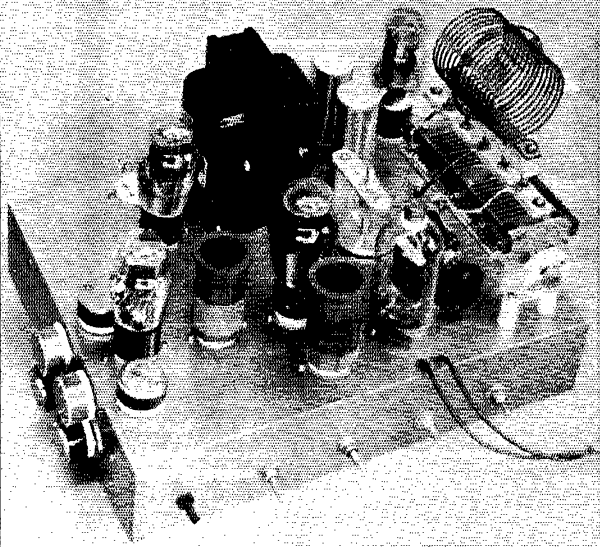
The transmitter chassis. Two leads at the lower right are connected to the meter on the transmitter panel.
