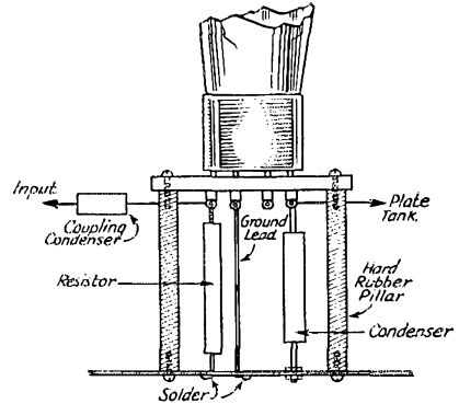
SOCKET ELEVATION
