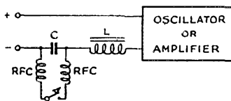
Fig. 3 — The general form of negative high-voltage keying, as used for all of the pictures in this story. Making the value of L larger introduces more lag to the start of the character, and increasing the value of C increases the lag (or "tail") at the end of the character.
