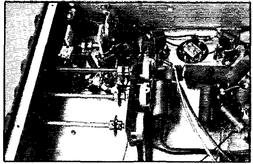
Close-up of the acorn first-detector and u.h.f. oscillator section underneath the chassis.
