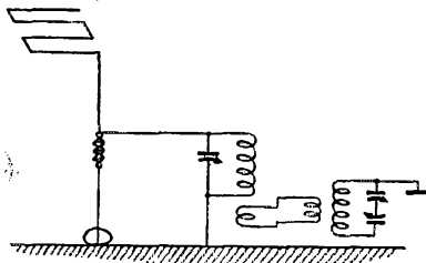
Fig. 9 — Sketch of the short vertical for 1.75 Mc. The total length of the wire is one-half wavelength. The folded portion at the top of the vertical section has a total length of one-quarter wavelength. The vertical portion is made as long as possible, while the remainder of the half wave is used as the lead to the transmitter.
