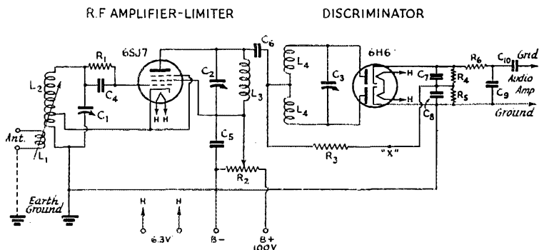
Fig. 1 — Circuit diagram of the two-tube r.f.-regenerative f.m. tuner.
