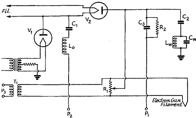
Fig. 3—Simplified schematic of the rectifier-doubler and filter. Terminal P_1 connects to the d.c. control amplifier ( P_1 in Fig. 4); P_2 is the lead from the driver oscillator; P_3 connects to the source of r.f. power which heats the electron-gun filament. V_1 and V_2 are special rectifier tubes (RCA-6132).
