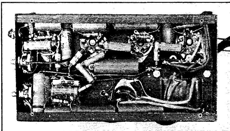
In this below-chassis view the sockets for the speech tubes are lined up along the bottom. Placement of parts is not critical; in this case, the layout was largely dictated by the necessity for finding room for the larger condensers.
