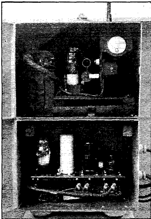
A 2½-meter emergency transmitter built chiefly from salvage parts. The upper compartment contains the r.f. unit and filament transformer, while the lower section houses the power and audio equipment. Interconnections are made through the cables at the right.
