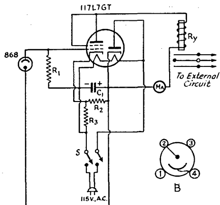
Fig. 4—Circuit diagram of the photocell relay.
