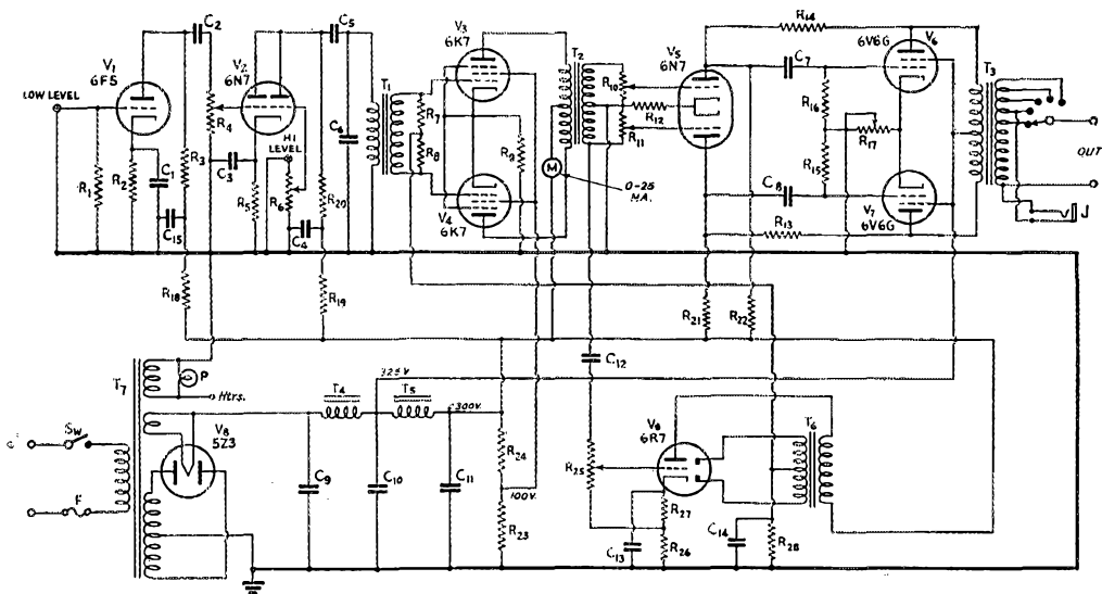
Fig. 1 — Circuit diagram of the peak-limiting recording amplifier. Audio voltage for the 6R7 control amplifier-rectifier is taken from the output of the push-pull 6K7 controlled stage, providing instantaneous a.v.c. action.
