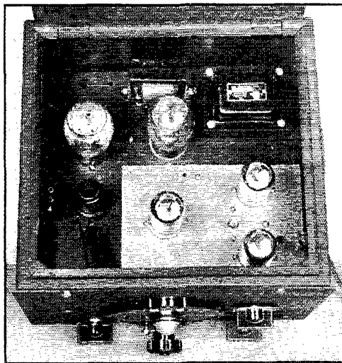
In this view of the receiver with the r.f. unit installed, the audio section is along the left edge of the chassis and the power supply is at the upper right. The cabinet is approximately 9\frac{1}{2} inches square and 7 inches deep.
