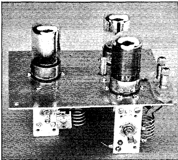
The r.f. unit, consisting of the mixer, high-frequency oscillator and superregenerative detector, is built on a small subchassis. The hole between the mixer tube and antenna binding-post assembly is for screwdriver adjustment of the i.f. transformer primary.
