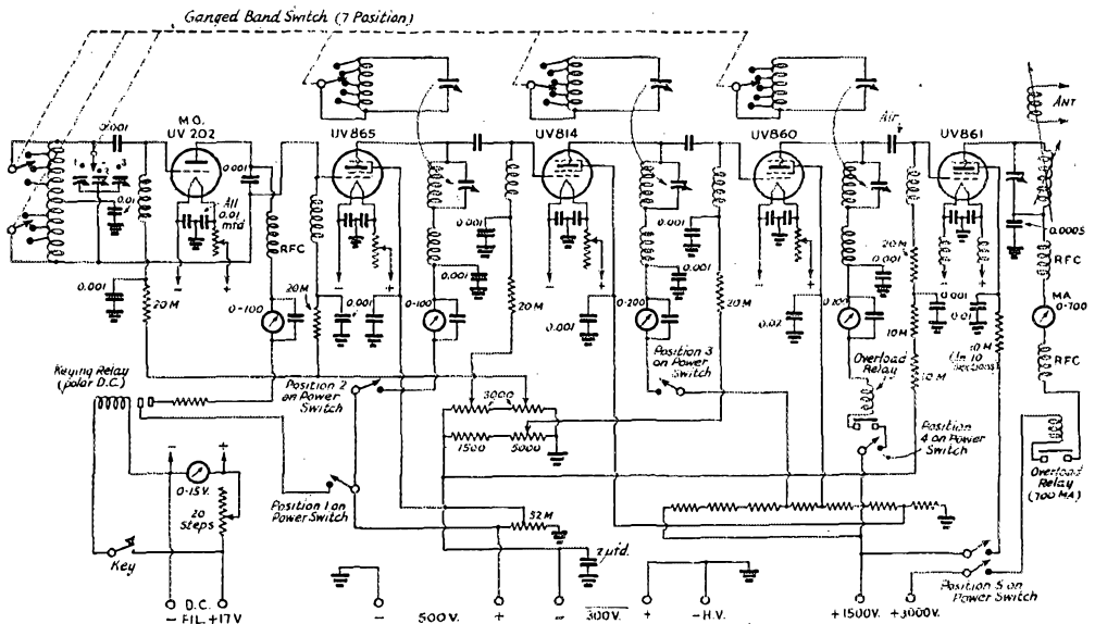
Schematic of the captured Japanese high-frequency transmitters, as traced by the author and W5JWV. The circuit as shown includes the modifications for c.w. operation described in the text. Contrast the obsolete tubes with the elaborate band-switching and control systems. Although Japanese made, the tubes were replicas of U. S. types.
