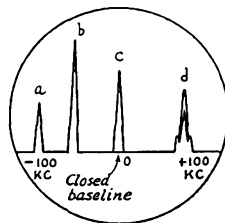
Fig. 1 — Typical signal patterns on the screen of the cathode-ray tube of the panoramic receiver. The peaks a and b indicate a c.w. signal or unmodulated carrier. The closed baseline of c indicates a rapidly keyed signal, while d 's irregular shape identifies it as a modulated carrier.
