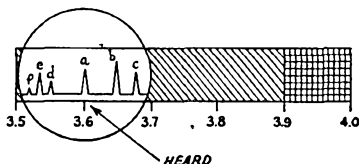
Fig. 3 — This is the same as Fig. 2 except that the receiver is now tuned to 3.6 Mc., the panoramic sweep now covering a range of 3.5 to 3.7 Mc.
