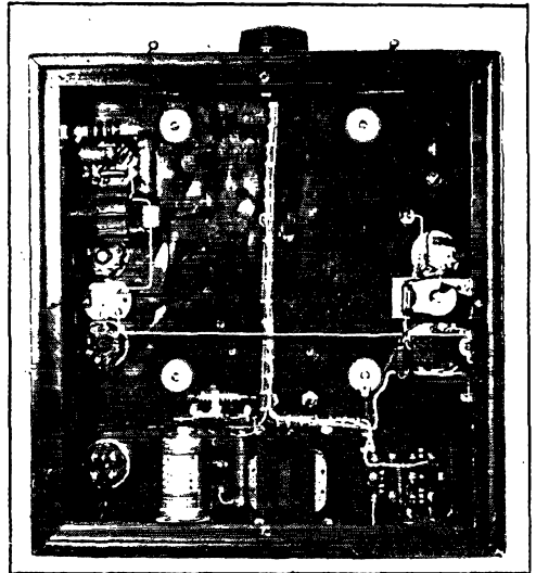
Bottom view of the v.f.o. rig. Grouping of parts in each circuit is shown. Power-supply components are at the top, the 6V6G doubler stage is at the left, and the 6J7 buffer is at the right. The four rubber grommets are at the corners of the oscillator box. A bottom cover is provided for the cabinet.
