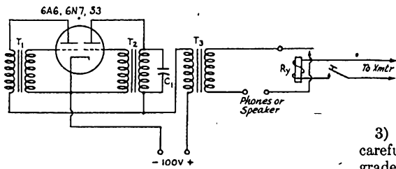
Fig. 3 — Dual-tone audio-oscillator keying monitor.
