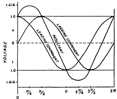
Fig. 9—Graph showing two voltages with a 90-degree phase difference and their resultant.
