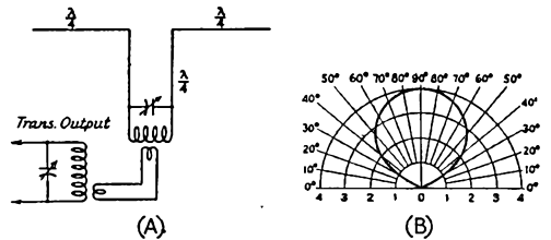
Fig. 4 — A — Half-wave antenna with quarter-wave tuned feeders and simple link coupling to the output stage. B — Pattern of vertical directivity.
