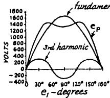
Fig. 4 — Resultant of the combination of fundamental and 20 per cent third-harmonic voltages.
