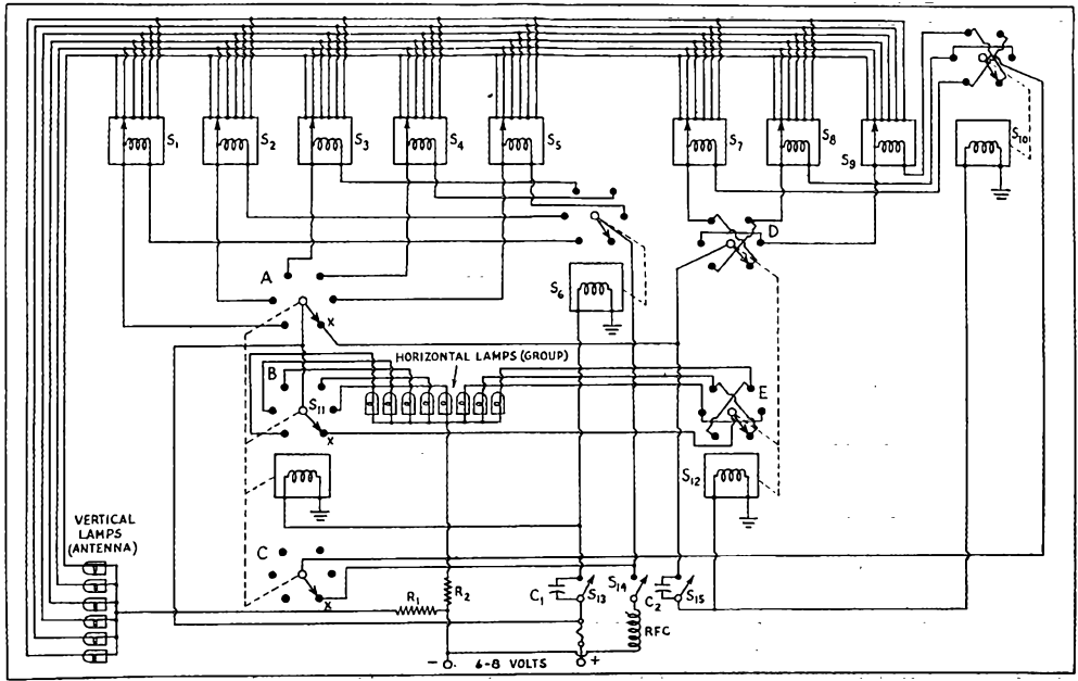
Fig. 2 — D.c. circuit of the third switch section. The negative terminal of the battery is grounded at the chassis. C_1, C_2 — 0.5 \mu f. RFC — 80 turns No. 16 wire on a 2-inch diameter form. R_1, R_2 — 15 ohms. A, B and C are sections of S_{11} , while D and E are sections of S_{12} (see Fig. 1).
