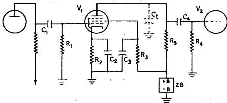
Fig. 1—Conventional RC-coupled amplifier stage.
