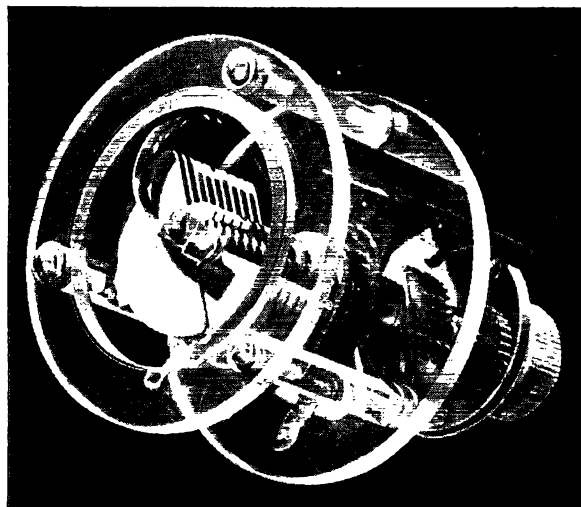
Rear-end view of the wide-range tank circuit covering the span from 65 to 380 Mc. The inductance is concentric with the inner edge of the rear supporting ring, which is made of plastic material.
