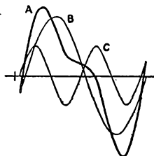
Fig. 14 — Complex wave after both component waves are delayed 30 degrees.
