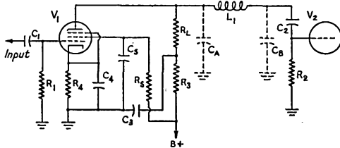
Fig. 20 — Typical series-peaking circuit.
