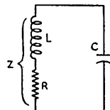
Fig. 7—Basic shunt-peaked network.
