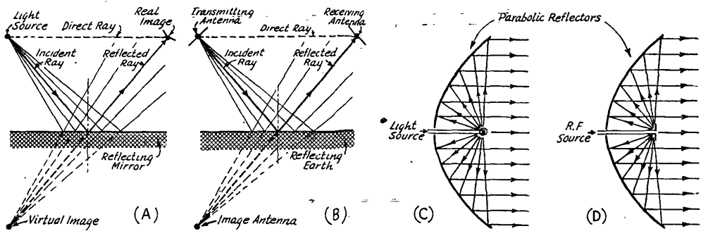
Fig. 2—The geometry of radiation is equally applicable to light rays and radio waves, provided the unit dimensions involved exceed a wavelength. A and B show the virtual image principle, long used in computing radiation patterns of antenna systems near ground as well as in optics. Parabolic reflectors are equally useful in directing a searchlight beam (C) or a radio beam (D). Any point on the parabola presents an angle such that waves radiated spherically from the point source in the focal plane are reflected as parallel in-phase plane waves.
