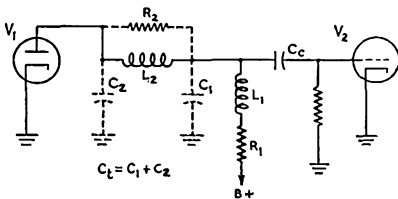
Fig. 11 — Combination-peaked stage.
