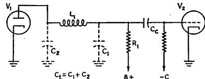
Fig. 9 — Series-peaked stage.
