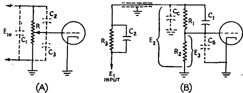
Fig. 18 — Attenuation systems. A — Uncompensated. B — Compensated.
