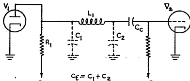
Fig. 8 — Series-peaked stage.
