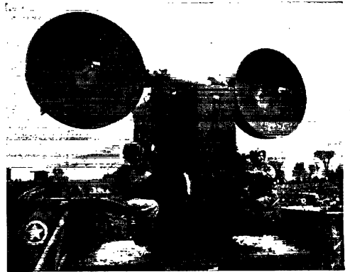
This radar equipment SCR-547, known as "Mickey Mouse" because of the shape of its antennas and used for aiming anti-aircraft guns, was installed near an anti-aircraft emplacement at Migano, Italy.
