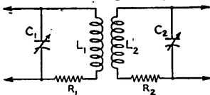
Fig. 1 — The double-tuned circuit.
