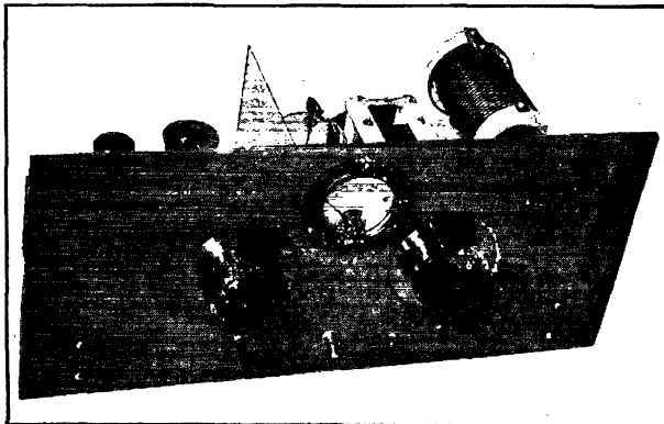
A two-tube medium-power transmitter. The panel is 3\frac{3}{4} inches high and the chassis measures 7 \times 17 \times 3 inches.
