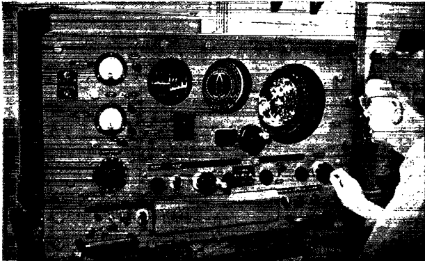
Above — Despite its inherent circuit complexity and numerous panel controls, the actual operating controls on the SG receiver are few. Glowing light pips and markers determine exact range and compass bearing of all objects in the region surrounding the ship. High-precision readings are obtained on auxiliary scan at left.
