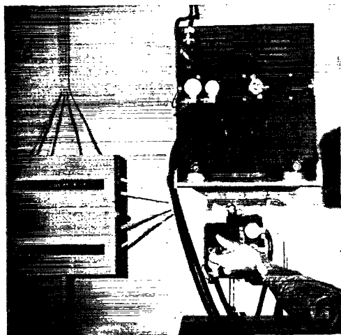
The flick of a switch on a shipboard IFF installation during a radar search determines whether a "pip" picked up on the radar scope is identifiable as "friend or foe."
