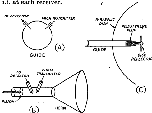
Fig. 1 — Details of a microwave communication system proposed by W3CHO. Placement of probes is shown at (A) and (B). A wave guide, terminated by a horn aperture and with a piston-type tuning device also is included at (B). Another type of termination, a parabolic dish, is shown at (C). An adjustable disc reflector also is detailed.
