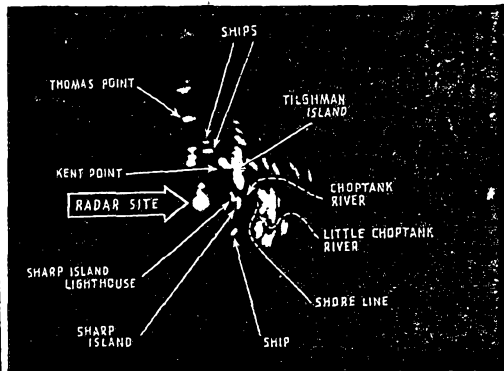
Below — Experimental radar equipment at NRL's Chesapeake Bay Annex made this "search" of the surrounding terrain. Lettered on the photographs of the PPI (Plan Position Indicator) screen are designations of points picked up by the radar pulse. Compare the two in terms of scale — the expanded screen view at the left exhibits increased distortion near the center. The pips converge when the range is widened, diverge when the range is lessened.
