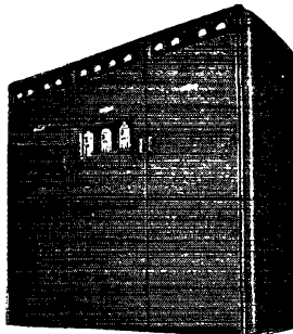
Collins 1000-C —Nominal power output: 2500 watts. Frequency range: 2 to 20 Mc. Additional a.f.-modulator & r.f. multi-channel sections available.
