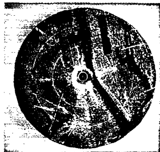
Below — Experimental radar equipment at NRL's Chesapeake Bay Annex made this "search" of the surrounding terrain. Lettered on the photographs of the PPI (Plan Position Indicator) screen are designations of points picked up by the radar pulse. Compare the two in terms of scale — the expanded screen view at the left exhibits increased distortion near the center. The pips converge when the range is widened, diverge when the range is lessened.
