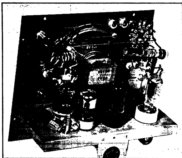
Rear view of the TR-4 showing the reduction in tank coil size for 144 Mc. and the filament chokes for the HY615.
