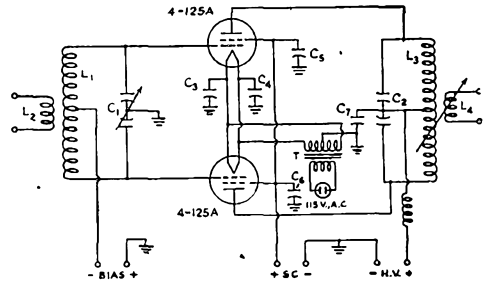
Fig. 1 — Circuit diagram of the high-power push-pull tetrode amplifier.
