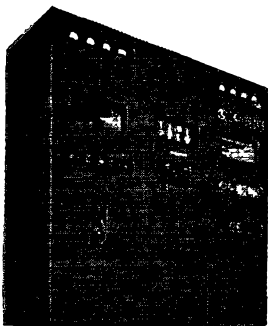
Collins 231D-13 — Nominal power output: 3000 watts phone; 5000 watts c.w. Frequency range: 2 to 18 Mc. Ten quick-shift frequencies.
