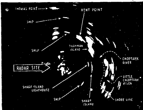
Below — Experimental radar equipment at NRL's Chesapeake Bay Annex made this "search" of the surrounding terrain. Lettered on the photographs of the PPI (Plan Position Indicator) screen are designations of points picked up by the radar pulse. Compare the two in terms of scale — the expanded screen view at the left exhibits increased distortion near the center. The pips converge when the range is widened, diverge when the range is lessened.
