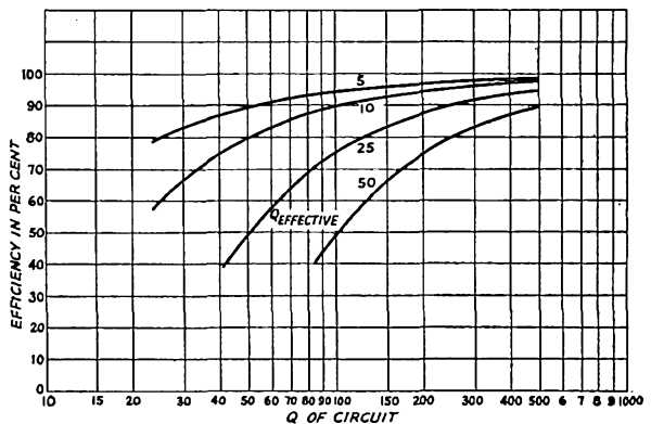
Fig. 12 — Curves showing final-amplifier tank-circuit efficiencies depending upon Q of circuit from Eq. (21).
