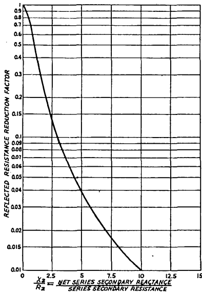
Fig. 10 — Chart showing reflected-resistance reduction as a result of detuning.
