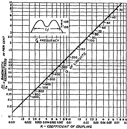
Fig. 4 — Values obtained from Eqs. (14) and (15) (level variation within pass-band 1 db.).
