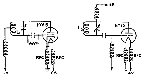
Fig. 1 — Partial circuit diagram showing the insertion of filament chokes.
