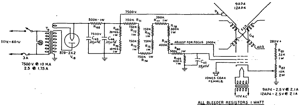
Fig. 7 — Circuit diagram of high-voltage power supply for the picture-reproducing tube.
