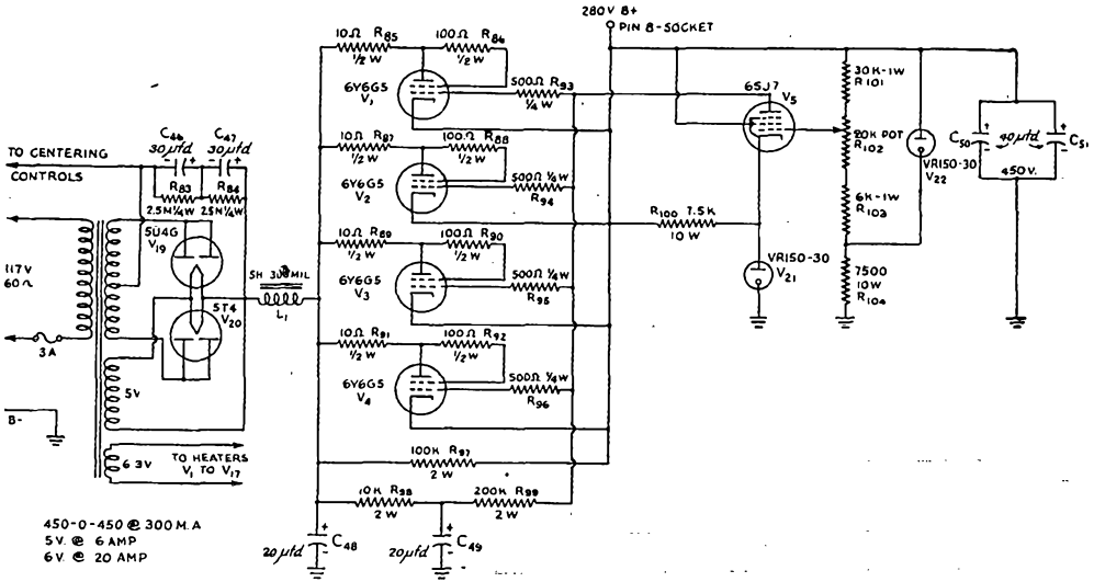
Fig. 6 — Wiring diagram of regulated power supply for the video and sync circuits.
