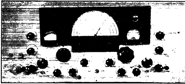
Control panel of the 21-tube receiver. It is made of Presdwood covered with pine-panelling wallpaper to match the walls of the operating room. The esutchcons are of crystalline-finished Presdwood, coated with India ink.
