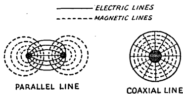
Fig. 4— Electric and magnetic field distribution in two-conductor transmission lines, looking into the lines through a cross section. The direction of propagation is either perpendicularly into or perpendicularly out of the paper, depending upon the relative directions of the electric and magnetic fields.
