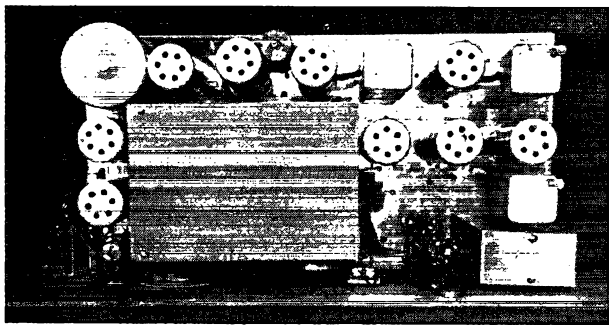
Plan view of the 21-tube superhet. The large compartment contains the h.f. tuning gang, tubes and associated by-pass condensers. The crystal-filter unit is in the lower right-hand corner, while the round shield can in the upper left-hand corner covers the microphone pre-amplifier. The i.f. strip runs along the top and down the right-hand edge of the chassis.
