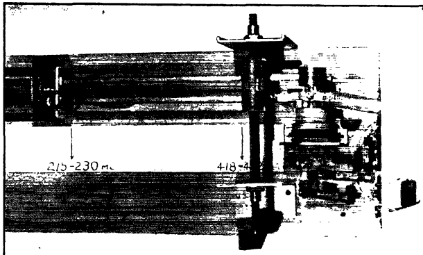
A close-up view of the tuning condenser also shows the details of the socket mounting and tube connections.
