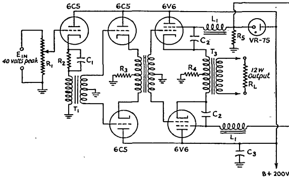
Fig. 9 — Circuit of a practical cathode-coupled amplifier.
