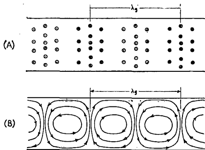
Fig. 13 — Instantaneous distribution of the electric field (A) and magnetic field (B) in a simple form of TE wave traveling through a rectangular guide. This is a view looking down on the wave, the side walls of the guide being represented by the horizontal lines. There is no component of the electric field directed along the guide (left to right) but the magnetic field does have such a component.
