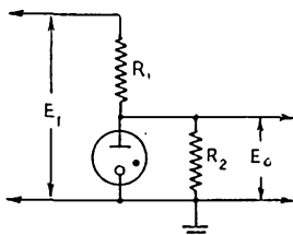
Fig. 1—Typical simple voltage-regulator circuit for VR-type tubes.
