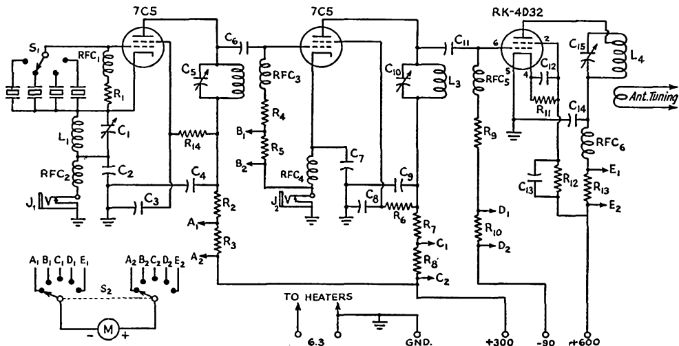
Fig. 1 — Wiring diagram of the 150-watt four-band transmitter.
