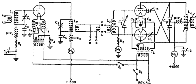
Fig. 1 — Schematic diagram of the 50-148-Mc., driver-amplifier using 35TG5.
