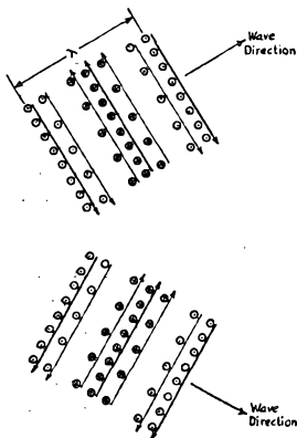
Fig. 12 — Another method of representing the two component waves of Fig. 9. Lines of electric force are represented by the small circles, the direction (perpendicularly into or out of the page) being indicated by dots or crosses. Relative field strength is indicated by the spacing of the circles. The associated lines of magnetic force are represented by the solid lines with arrowheads, with relative field strength indicated by the weights of the lines (still another method of portraying field properties!).
