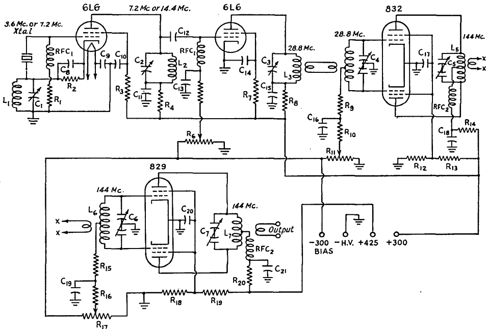
Fig. 2 — Circuit diagram of a 144-Mc. transmitter operating from a 3.6- or 7.2-Mc. crystal.
