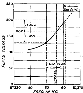
Fig. 2 — Plate voltage vs. frequency characteristic of a 7C5 self-excited oscillator under limited amplitude modulation.
