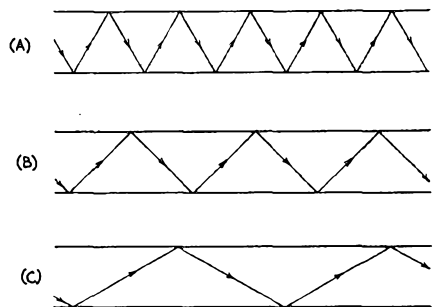
Fig. 11 — The three drawings in this figure correspond to the three in Fig. 10, and show the path taken by a component wave in traveling through the guide. The shorter the wavelength, the fewer reflections from the side walls in a given length of guide.
