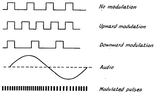
Fig. 2 — A pulse-modulation system using constant pulse length and varying the repetition rate in proportion to the modulation amplitude.
