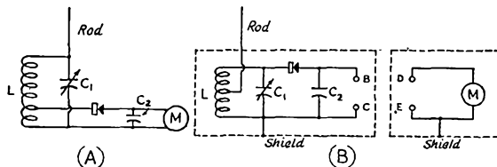
Fig. 3 — Field-strength meters using crystal detectors.
