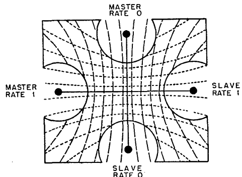
Fig. 7—Ideal layout for two pairs of SS Loran stations, showing good crossing angles and long base lines. The circles enclose "forbidden" areas of low accuracy.
