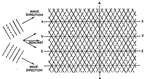
Fig. 9—The fields of two traveling waves add at any point in space to give a resultant at that point having an amplitude and direction dependent upon the amplitudes and directions of the two component waves. This drawing represents a space distribution for a single instant of time. The two wave components, assumed to have equal amplitudes, are shown at the left, with the direction of propagation indicated. The resultant wave direction is shown by the small drawings between. Along lines such as XX, YY and ZZ the resultant amplitude always is zero, giving rise to standing waves in space.
