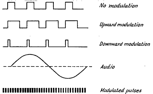
Fig. 1 — A representation of a pulse-modulated signal in which the repetition rate is held constant and the pulse length is changed in proportion to the modulation amplitude.
