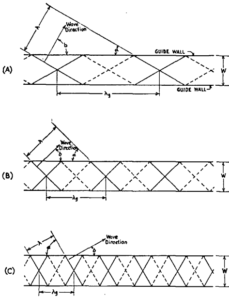
Fig. 10 — The smaller the wavelength in comparison with the cut-off wavelength of a guide, the smaller is the angle at which the wave strikes the side walls. In (A) the wavelength is close to the cut-off wavelength; in (B) a shorter wavelength is represented, and (C) shows the effect of making the wavelength still smaller. The width, W , of the guide is the same in all three cases. The wavelength in the guide, \lambda_g , always is greater than the free-space wavelength, but the ratio becomes smaller as the free-space wavelength, \lambda , is decreased.
