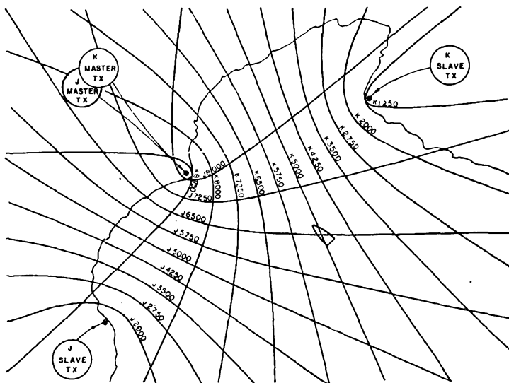
Fig. 5 — How two pairs of Loran transmitters furnish a fix for a ship.
