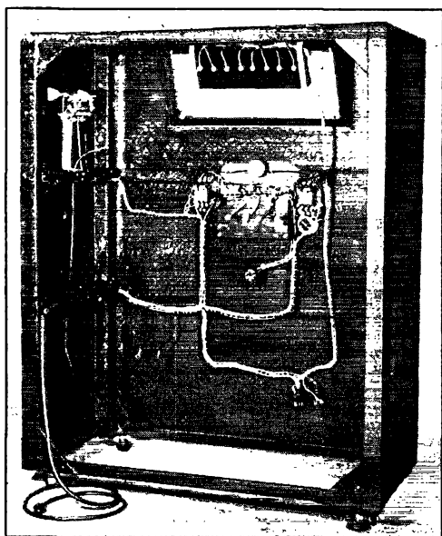
A rear view of the cabinet with the chassis removed, showing the antenna relay on the left-hand wall and the plug-in power cables.
