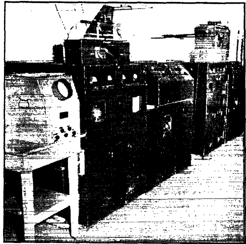
Official photograph, Royal Canadian Navy. The Loran transmitters at the Baccaro installation.
