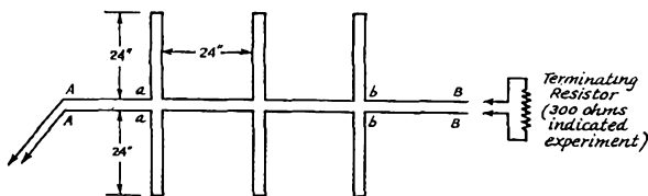
Fig. 2 — Schematic representation of the Series-phase Array. Line sections Aa and Bb may be eliminated if desired.
