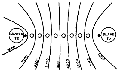
Fig. 4 — Hyperbolic lines of constant time difference with arbitrary numbers assigned.
