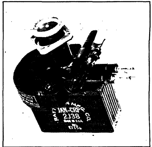
The 2J38 is a "compact" lower-powered magnetron of the package type that was used extensively in aircraft radar. The output fitting is for coaxial line.
