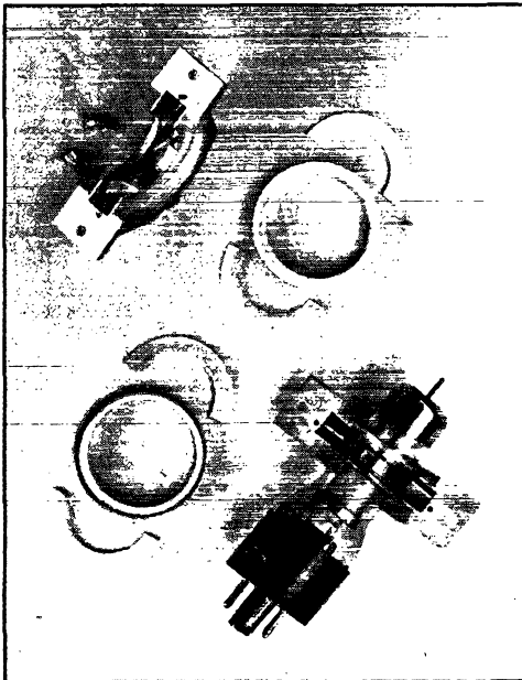
The local oscillator tube used in 3000-Mc. radar receivers, the 2K28 reflex klystron. The resonant cavity makes connection to the copper discs midway along the glass part of the tube. The other half of the disassembled cavity also is shown in this view.
