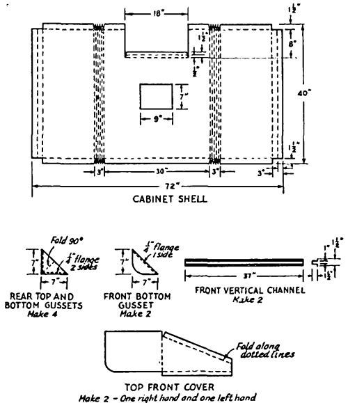
Fig. 1. — Details of the cabinet shell and reinforcing members. The material is 20 gauge cold-rolled steel.
