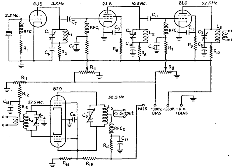
Fig. 3 — Circuit diagram of a 50-Mc. transmitter controlled by a 3.5-Mc. crystal.
