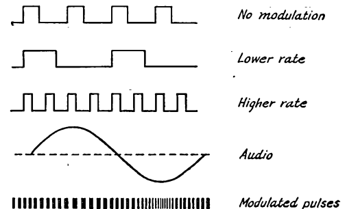
Fig. 3 — Maintaining the duty cycle constant results in a pulse-modulation system in which the repetition rate is proportional to the modulation amplitude, and the rate of change of repetition rate is proportional to the modulation frequency.
