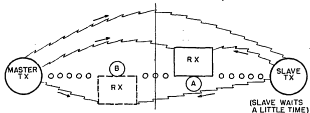
Fig. 3 — With a time delay between the Master and Slave transmissions, a receiver at A measures a smaller time difference between arrival of signals than does a receiver at B.
