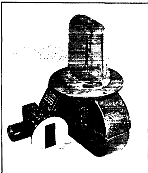
A "package-type" magnetron, in which the magnet is integral with the tube. The 2J55 operates at 9400 megacycles (3.2 centimeters). The over-all height of the tube is six inches.
