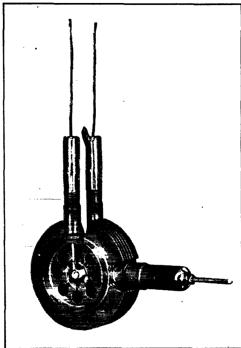
The real "works" of a 10-cm. magnetron, showing the eight cavities surrounding the cathode and the "strapping" of alternate cavities. The cathode is supported only by the heater leads coming in on either side of the cavities.
