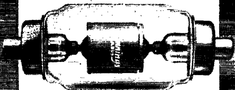
C-COCONUT, 50 mmfd., 50,000 Peak Volts, 60 Amps. Overall Length 8\frac{1}{2} " Long, 3" Diameter.
