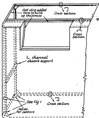
Fig. 2. — Assembly details of the transmitter console. The pieces are assembled with small rivets and then spot welded.
