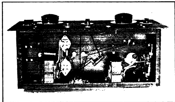
Under-chassis view of the 35TC driver-amplifier. Separate filament transformers are used for the two stages. The driver tube socket with its two filament r.f. chokes is at the right.
