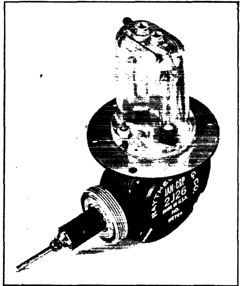
A 300-kilowatt magnetron, the 2J26. The output connection projects from the seal in the foreground. The pyrex bowl on top protects the cathode and heater leads and provides a mounting for the terminal jacks.
