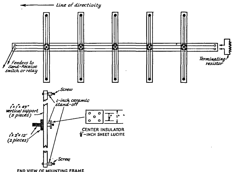
Fig. 1 — The experimental model of the Marconi-Franklin Series-phase Array. Any number of vertical sections may be used. The folded portions should be spaced as closely as possible — the \frac{1}{2} -inch spacing shown is a convenient form. The array is unidirectional, toward the transmitter end.
