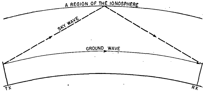
Fig. 6—A longer time is required for the sky-reflected wave to reach the receiver than is taken by the ground wave, because of the longer path.
