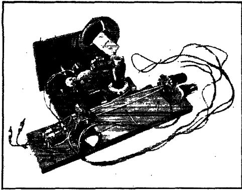
Rear view, including the high-dielectric-strength South-corn pine matches. (The Lecher-wire support mechanism probably is more easily identified in this than in the front view.)
