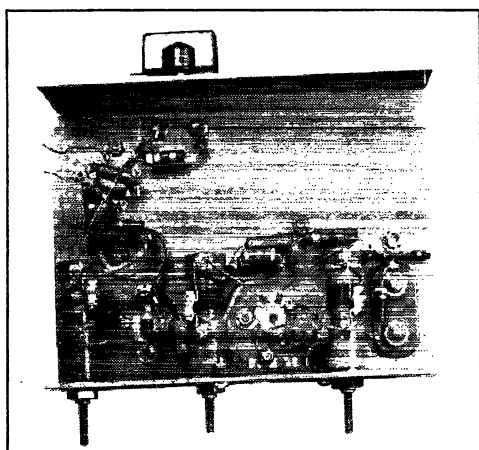
Bottom view of the three-tube 2-meter converter. Note the fixed-tune tank circuits mounted along the back edge of the chassis. The two short leads at the upper left connect to the antenna terminals of the One-Ten receiver.
