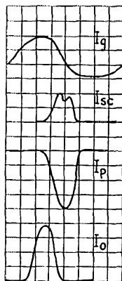
Fig. 2—Tuning characteristics of an 807 with less than adequate excitation.
