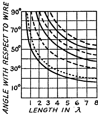
Fig. 3— Graph showing positions of maximums (solid lines) and nulls (dashed lines) as a function of antenna length in wavelengths. The dotted line shows the angle at which maximum phase addition occurs.
