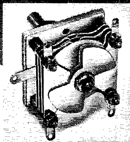
PL-6113 (Type ER-14-BF/S) Range: 14-11 mmf. (approx.) (Minimum capacity loaded by circular rotor plates — for a High "C" circuit.) Amateur Net: $2.40
