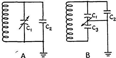
Fig. 2—In this diagram C_2 represents the input capacitance of the tube used with the tuned circuit. The effect on minimum capacitance of the circuit is reduced in the split-stator circuit at B because C_2 is in series with one section, C_3 , of the tuning condenser.
