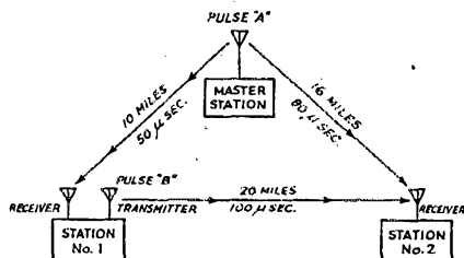
Fig. 1—A block diagram showing the principle of selective pulse communication. Master Station sends a special pulse which is received at both No. 1 and No. 2. No. 1 relays this pulse and it is tuned in by opening a "gate" in the receiver at No. 2 at the proper instant.
