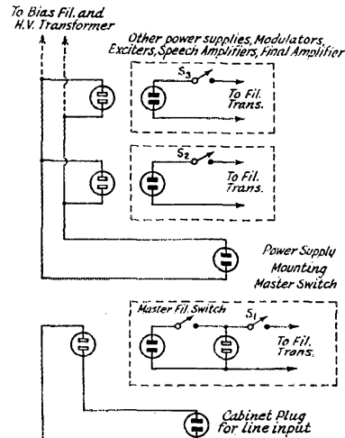
Fig. 1 -- The filament circuits are controlled by one Master Filament Switch mounted on one of the power supplies. The individual filament switches, S 1 , S 2 and S 3 , might be omitted on r.f. units that are used all of the time, but they are recommended on equipment that is not always in use, such as speech amplifiers and modulators. Plugs are shown with solid contacts; open contacts indicate receptacles.
