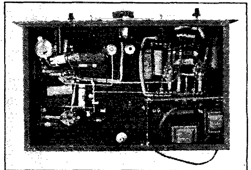
Small components are placed underneath the chassis. The filter chokes are in the shielding compartment in the upper left-hand corner.
