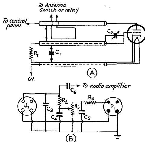
Fig. 2 — A shows the schematic diagram of the receiver proper. B is the superregenerative receiver control panel.
