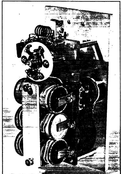
The r.f. circuit components are arranged in a compact group on the polystyrene subpanel at the top. The antenna makes contact with the terminal of the trimmer-type coupling condenser.
