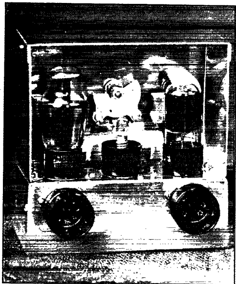
Rear view of the v.f.o. shows its compact arrangement. The coils are mounted on the rear of the chassis which must be kept clear of other units when in use.
