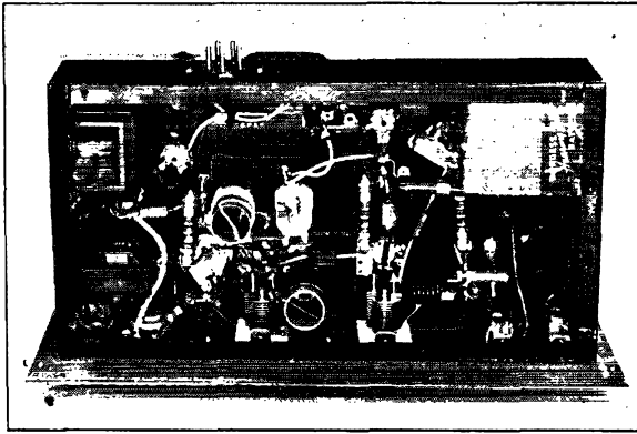
Bottom view of the mobile rig. At the left center are the interwound coil and tuning condenser which are part of the oscillator filament circuit. Audio components are at the left, with oscillator and multiplier plate circuits near the front panel.
