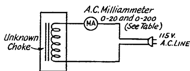
Fig. 1 — Using an a.c. milliammeter to measure current for determining inductance.
