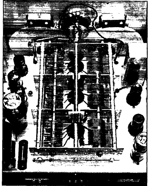
A top view of the HQ-129-X with the dust cover removed from the tuning-condenser assembly to show the main-tuning gang (right) and the bandspread condensers. The antenna trimmer condenser is in the center.
