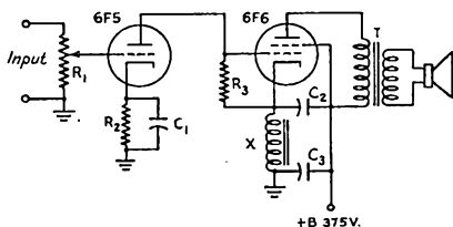
Fig. 1 — Direct-coupled amplifier requiring a minimum of parts.
