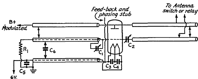
Fig. 1 — Schematic diagram of the 420-Mc. oscillator.
