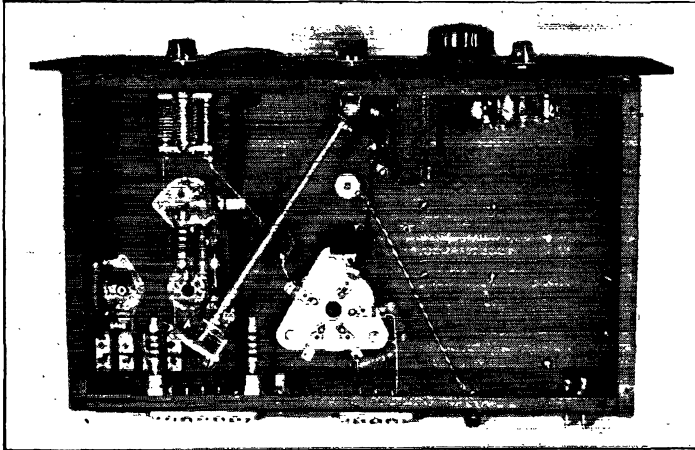
Bottom view showing the arrangement of parts under the chassis. Mounted off the rear edge of the chassis are the oscillator (left) and amplifier (right) grid chokes. The oscillator plate choke is above. The condenser under the crystal-switch control shaft is the coupling condenser, C_8 . The oscillator tuning condenser, C_2 , the 6.3-volt filament transformer and the metering switch are along the front edge of the chassis.
