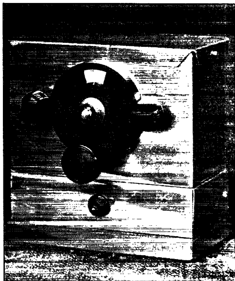
Front view of VE4ANQ's v.f.o.
