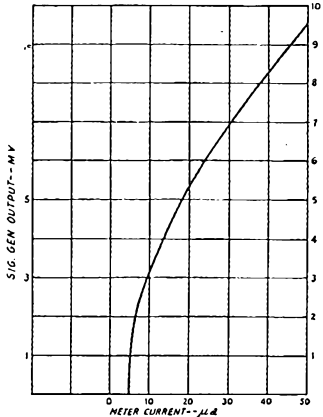
Fig. 2 — Response curve of the v.h.f. f.s. meter in terms of millivolts input and microamperes deflection.
