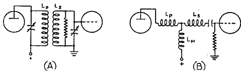
Fig. 2 — (A) Transformer coupling. (B) Common-impedance coupling.
