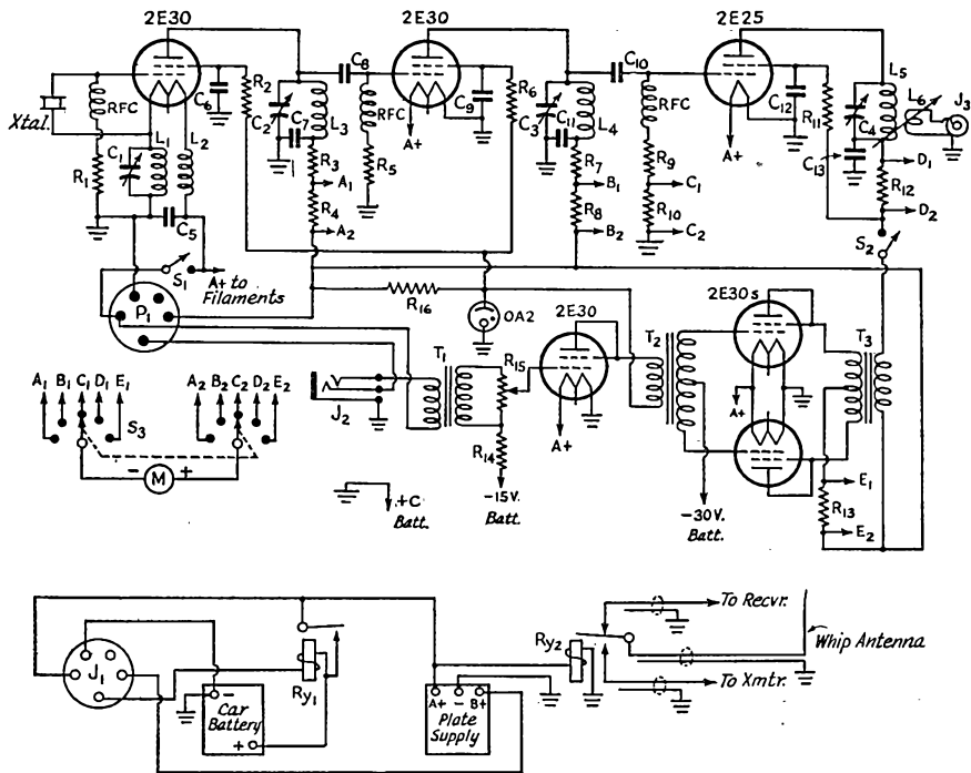
Fig. 1 — Wiring diagram of the mobile rig for 6 and 10 meters.
