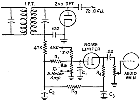
Fig. 1 — Noise-limiter circuit of the HQ-129-X.
