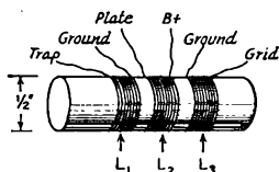
Fig. 5—Details of windings for the circuit of Fig. 4. Coils are spaced \frac{1}{8} inch.
