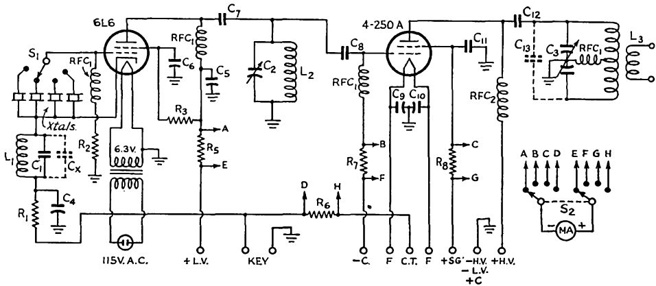
Fig. 1 — Circuit diagram of the two-stage high-power transmitter.
