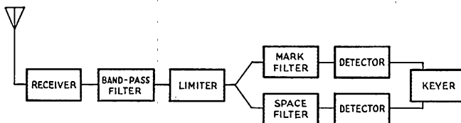
Fig. 1 — Block diagram of representative receiving system for frequency-shift keying.
