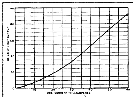
Relationship between light output and current in the R1130B (1B59)
