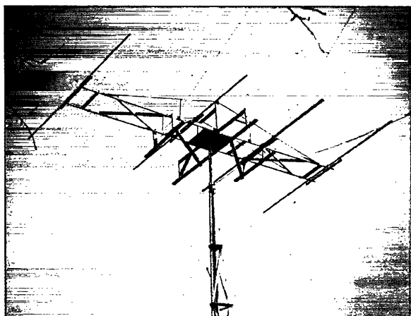
The 4-element rotary array for 50 Mc. installed atop its steel tower. The frame extending below the main framework serves as a rotating device. The array frame is mounted on a pipe flange, to which is fitted a length of pipe which serves as a vertical support.
