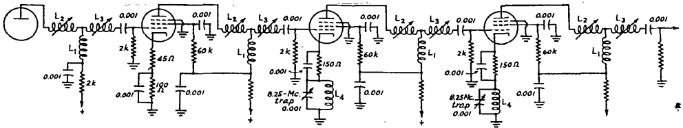
Fig. 6 — Circuit for an i.f. amplifier with a 4-Mc. bandwidth.
