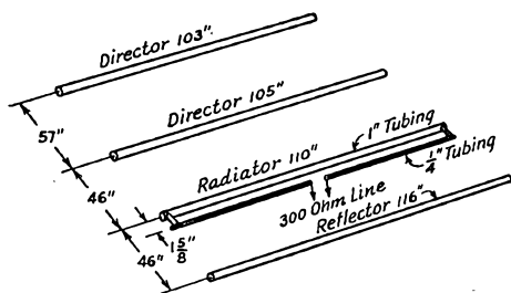
Fig. 2 — The spacing and length of the elements in the 50-Mc. array were arrived at experimentally. Dimensions given are for 50.5 Mc.
