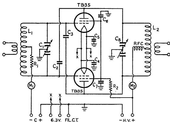
Fig. 1 — Circuit diagram of the amplifier.
