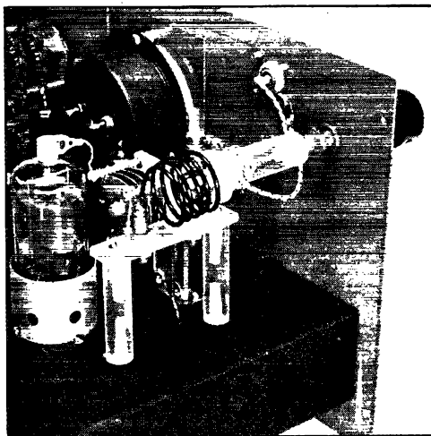
Detail photo of the 2E25 final stage, showing method of coupling to the antenna. The coupling coil, wound on a polystyrene rod, is adjustable from the front panel. The plate coil is mounted by means of G.R. plugs.
