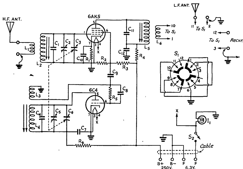
Fig. 1 — Circuit diagram of the 50-Mc. converter.
