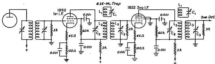
Fig. 4—Circuit for two-stage amplifier with 2.5-Mc. bandwidth.
