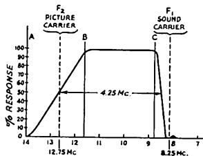
Fig. 1 — Selectivity curve of television i.f. amplifier.
