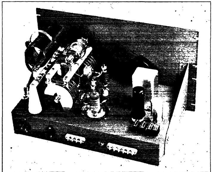
◆ Rear view of the two-stage high-power transmitter, showing the vacuum-type padding condenser in place on top of the tank condenser. ◆
