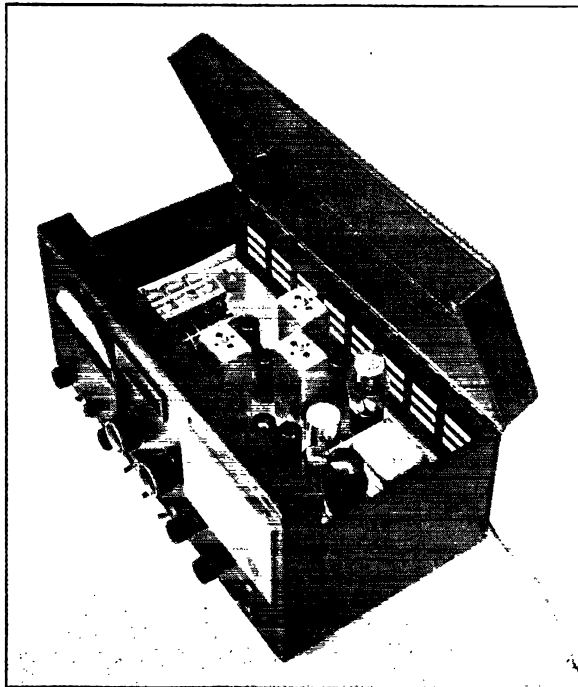
A glimpse inside the S-40. The linged cane-metal lid not only provides plenty of ventilation but the design is such that it is easy to get at the parts on the chassis.
