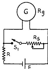
Fig. 3 — Measuring the resistance of a meter by utilizing the meter itself as the current indicating device. See text for component values.
