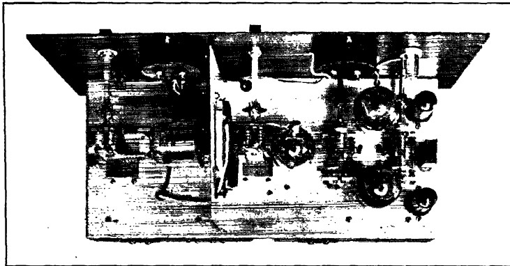
◆ A plan view of the 144-Mc. crystal-controlled transmitter. The set is push-pull throughout, with all frequency multipliers operating as triplers. The crystal oscillator, using 6AC7s, is at the right, the following stages (progressing to the left) being the 6L6Gs as first tripler, 815 as second tripler, and 829 final amplifier. ◆
