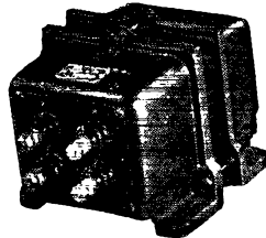
350 WATT MODULATION TRANSFORMER Brand new units as used in the BC-610 transmitter. Primary for class "B" 100-TH Modulators. Secondary 8300 ohm class "C" load at 250 ma. Special, Net..... $21.50
