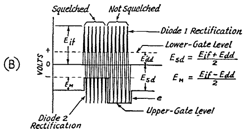
Fig. 5—(A) Basic double-gate A.M.D. circuit. (B) That portion of the signal represented by E_{if} - E_{da} is fully modulated by E_M . E_{if} = peak i.f. voltage; E_{da} = detector threshold level (lower gate); E_M = peak a.f. modulating voltage; E_{da} = squelch-diode d.c. delay bias; E_{da} = detector-diode d.c. delay bias (= E_{da} ); e = squelch-diode instantaneous delay bias.
