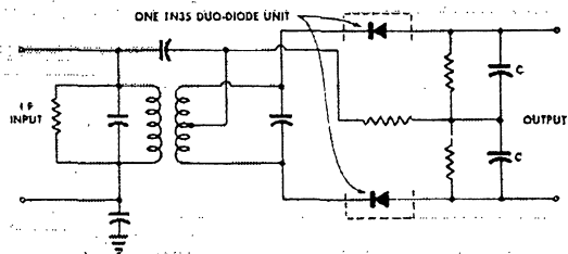
The 1N35 in frequency discriminator circuit
