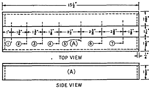
Fig. 2 — Working plan of the wooden chassis for the transmitter. (The chassis for the power supply is constructed in the same manner, and its dimensions are the same except for the length, which is 9\frac{1}{4} inches instead of 15\frac{1}{2} inches.)
