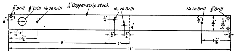
Fig. 2—Dimensional drawing of the 141-Mc. tank inductance before bending. The material is ¼-inch copper strip.
