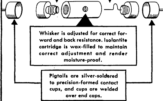
CONSTRUCTION DETAILS OF THE 1N35
