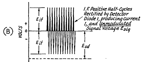
Fig. 3 — (A) Same as Fig. 2-A but with d.c. delay bias E_{ad} added to squelch-diode 2 only. (B) Operational diagram showing how squelch-diode 2 is prevented from rectifying the i.f. negative half-cycles so long as E_{ad} is larger than E_{if} .
