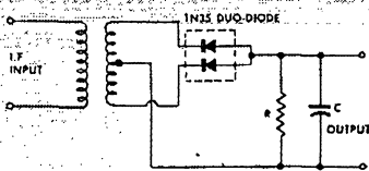
Full wave rectifier second detector circuit
