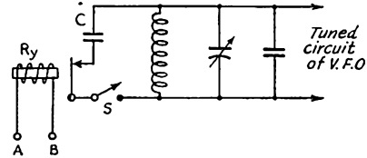
Fig. 3 — Elimination of drift during VFO stand-by. The relay (operated by a source of power available when the transmitter is on) removes the padding condenser C from across the VFO which then returns to the desired operating frequency. When the transmitter is turned off the relay closes and the padder lowers the VFO frequency sufficiently to move it out of the way of the incoming signal in the receiver.
