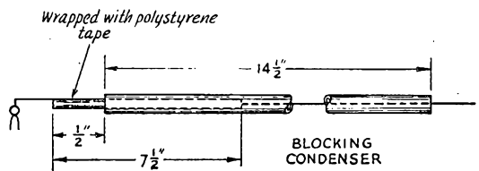
Fig. 4 — Construction of the plate blocking condenser. The inner tube has a diameter of \frac{3}{8} inch and, like the resonant line, should be silver-plated.
