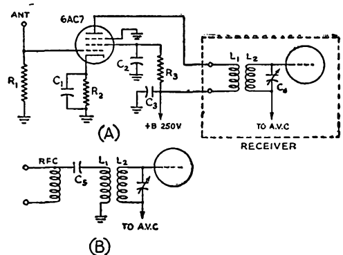
Fig. 4 — This untuned preselector requires only a few components and a 6AC7 yet it will improve the performance of the ordinary variety of communications receivers having no preselection. An alternate method of coupling to the receiver is shown in (B) where an r.f. choke replaces L_1 in the circuit shown in (A) and is capacity coupled to the antenna winding of the receiver.
