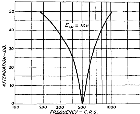
Fig. 4 — Response curve of the selective audio amplifier shown in Fig. 1.
