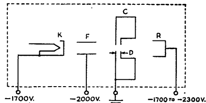
Fig. 3 — This diagram illustrates the basic construction of the Z-668 reflex oscillator tube.
