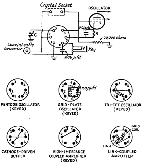
Fig. 2 — Six different oscillator-circuit arrangements are available in this oscillator socket layout worked out by W8UPS. Condenser C must be large enough (100 to 250 \mu\text{fd.} ) to resonate the Tri-tet coil or the link-coupled amplifier grid coil. The value of R will vary with various tubes and should be the normal cathode resistor for the tube selected.
