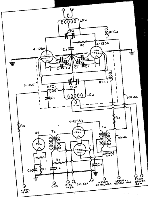
Typical High-Level Modulated R-F Amplifier Circuit. (Note: Separate screen winding not required on modulation transformer.)
