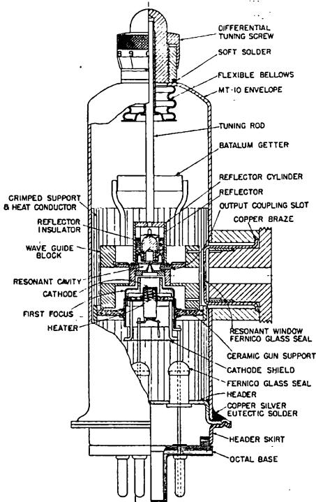
Fig. 4 — Cross-sectional drawing showing the construction of the Z-668 tube.
