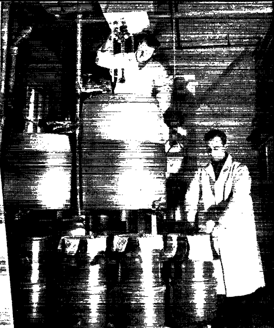
First floor of Hytron chemical precipitation system. Note the flow meter, precipitation tanks, and ceramic vacuum filters. Spotless cleanliness is vital to avoid contamination of carbonates precipitated for cathode coatings.
