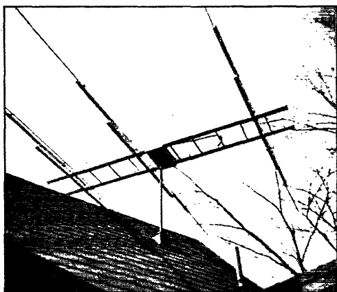
The ladder-supported three-element beam. The pipe mast projects through the roof and rests on a bearing made from pipe flanges. A housing of larger pipe, inside the attic, serves as a sleeve in which the mast can rotate.
