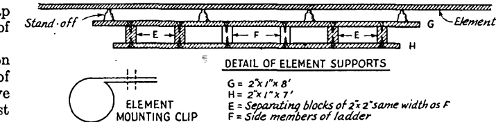
Fig. 3 — The element supports. These mount at right angles to the adder (indicated in cross-section at "F").
