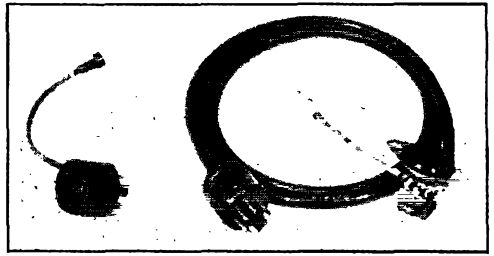
The adapter plug and extension cable. The 6H6 socket, at the right, should be grounded at a convenient point on the receiver near enough to the second-detector socket to permit joining the pin-jack and prod.
