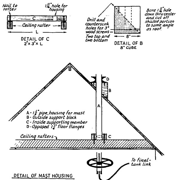
Fig. 1—Sketch showing the attic housing, with the mast protruding through the operating-room ceiling and automobile steering wheel for turning the antenna. Dimensions of the housing and mast will depend on the individual location.
