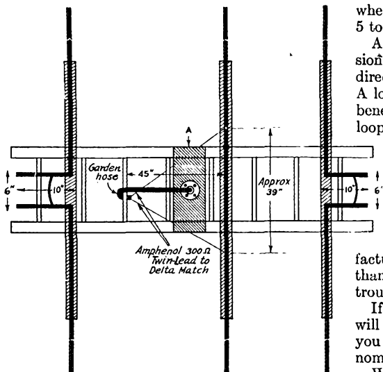
Fig. 4 — Top view of the assembled beam, showing the method of running the 300-ohm transmission line through garden hose for protection against weather and abrasion.
