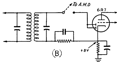
Fig. 6 — Diode-detector circuit commonly used in receivers. The circuit at A uses a separate diode rectifier while that at B uses a combination diode-triode tube. In the latter case, the diode plates, in the absence of signal, are given a positive voltage with respect to the chassis by the voltage drop across the cathode resistor. This bias must be compensated in the adjustment of the A.M.D. adapter.
