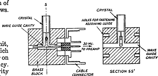
Fig. 2—Cross-section of the crystal mixer.
