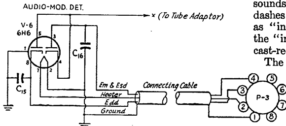
Fig. 5 — Circuit diagram of the A.M.D. diode adapter and connecting cable to main unit. C_{15} — 0.01- \mu d. mica. C_{16} — 0.004- \mu d. mica.
