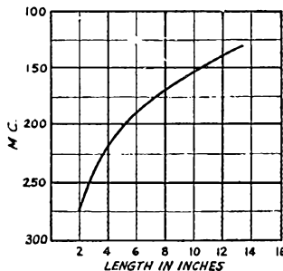
Fig. 6 — Oscillator frequency as a function of line length. This curve is indicative only, since the exact frequency will depend upon the individual tube and line.
