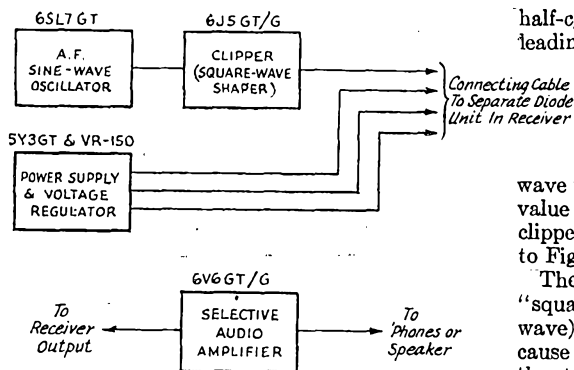
Fig. 2 — Block diagram of the main A.M.D. adapter unit.
