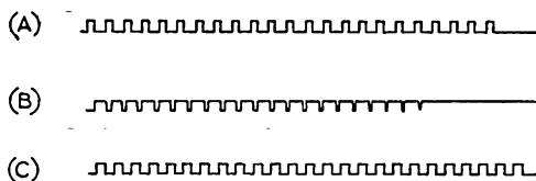
(A) Dot contacts too far apart. (B) Dot contacts too close. (C) Dot contacts correctly adjusted.
