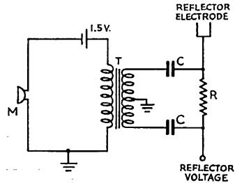
Fig. 5 — Circuit for frequency modulating the Z-668 oscillator.
