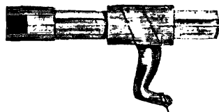
Phantom View showing how tapered shank of Nylon needle fits into tapered hole in Nylon chuck.
