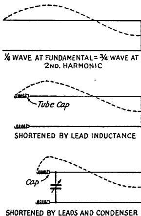
Fig. 1 — Current distribution at the second harmonic along a "quarter-wave" line. If peak current occurs at or near the tube cap, as shown in the bottom sketch, overheating and consequent melting of the solder can occur.
