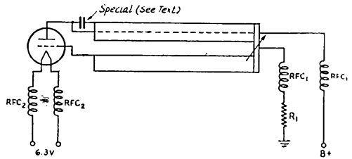
Fig. 3 — Circuit diagram of the 140-250-Mc. oscillator shown in the photograph. The line is constructed of \frac{1}{2} -inch tubing, silver-plated, the grid tube being 15 inches long and the plate tube 14\frac{1}{2} inches long. Length in use is adjusted by the shorting bar shown in Fig. 5. Center-to-center spacing of the conductors is 1 inch. R_1 — 5000 ohms, 10 watts. RFC_1 — 40 turns No. 28 spaced to occupy a length of 1\frac{1}{8} inch on \frac{1}{4} -inch diameter form. RFC_2 — 27 turns No. 18 enameled closewound on \frac{3}{8} -inch diameter form.
