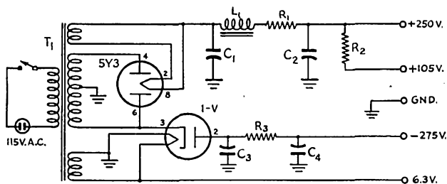
Fig. 2 — Power-supply wiring diagram.
