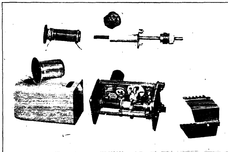
A view of the oscillator with the shields removed to show the internal arrangement. The disassembled permeability-tuned coil and the ceramic tank condenser are shown at the top.
