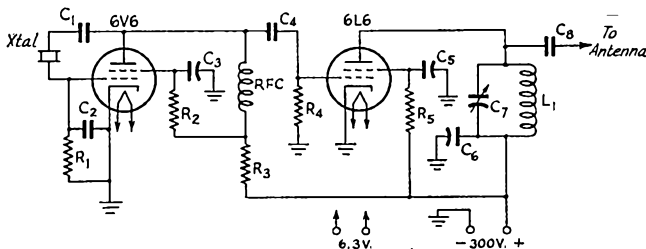
Fig. 1 — Single-control oscillator-amplifier combination.
