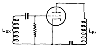
Fig. 1 — Fundamental oscillator circuit.
