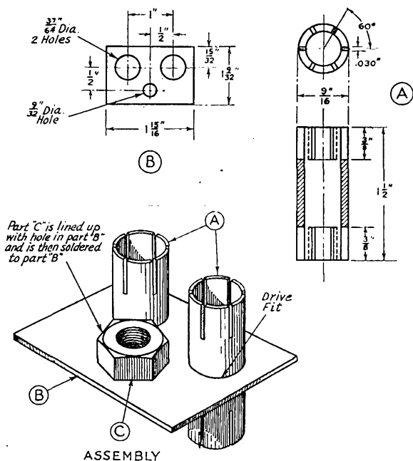
Fig. 5 — Shorting-bar details. "C" is a \frac{1}{4} -inch brass nut serving as part of the drive mechanism. It is engaged by a threaded fiber rod, mounted as shown in the photograph, for knob tuning.
