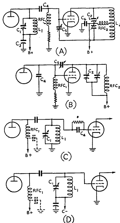
Fig. 2 — (A) Usual capacitance-coupled triode amplifier circuit with insulated plate-tank condenser. (B) The resulting low-frequency parasitic circuit. (C-D) Circuits which eliminate low-frequency parasitic grid tanks.
