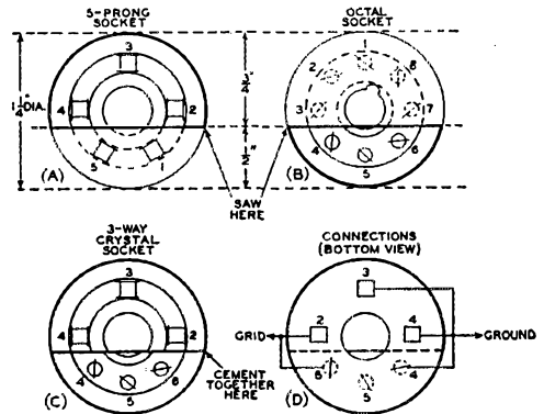
Fig. 4—Method of constructing a 3-way crystal socket from portions of a 5-prong socket and an octal socket. The two are cut as shown in A and B, and are cemented together as shown in C. The socket connections to permit use of any of the three popular sizes of crystal holders are shown in D.
