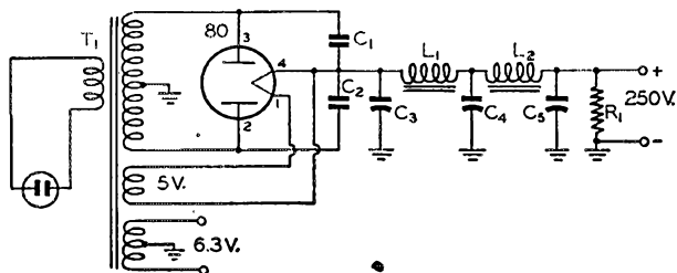
Fig. 2 — Circuit diagram of the receiver power supply. C 1 , C 2 — 0.002- \mu fd. mica. C 3 , C 4 , C 5 — 8- \mu fd. 450-volt electrolytic. R 1 — 50,000 ohms, 5-watt wirewound. L 1 , L 2 — 10-henry 50-ma. choke. T 1 — Power transformer, 240-0-240 volts, 50 ma.; 5 v.; 6.3 v.
