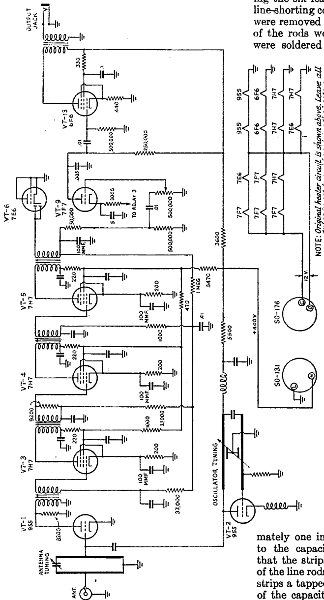
Fig. 2—Schematic of the receiver as converted for 420 Mc. Two stages of audio, employing tubes already in the unit, have been added. The oscillator lines are lengthened (see photo) and a.v.c. is incorporated.
