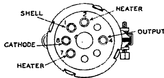
Fig. 3 — Detail drawing of the 723A/B s.h.f. oscillator tube. Tube potentials are as follows: heater — 6.3 volts, a.c. or d.c.; cathode — 0; resonator (shell) — 300 volts d.c., positive; repeller (cap) — 20 to 300 volts d.c., negative.
