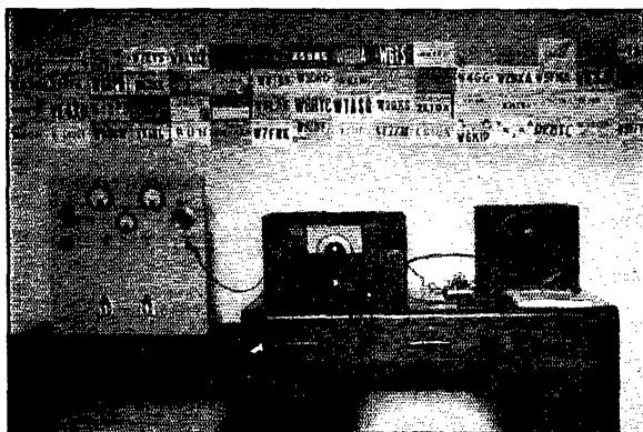
◆ The photo last month of CR9AN showed only one-half of his shack. Here is the other side with the rig that is now doing the business. The transmitter is a 6L6 driving an 813, and crystal switching is used when quick QSY is required to get out from underneath the DX hogs. The receiver is an NC-100A and the antenna is a single-section W8JK . Those cards on the wall are all a result of the QRP work, however.
