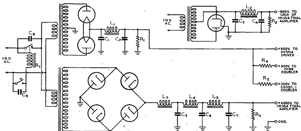
Fig. 2 — The break-in primary keying used at WILZ which gives lag-free T9 keying. The large amount of filter in the final amplifier supply is not necessary — it was included only to prove that any amount can be used without introducing lag.
