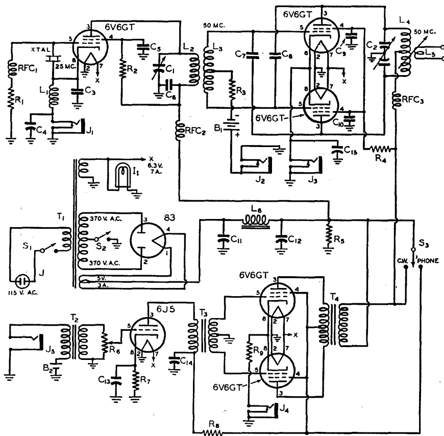
Fig. 1 — Circuit diagram of the six-meter transmitter.
