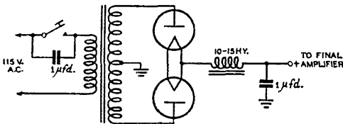
Fig. 1—Primary keying first used at W1LZ. It is impossible to obtain crisp keying and a T9 signal when only the final-amplifier supply is keyed.
