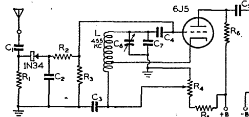
Fig. 1 — An untuned keying monitor that may be installed inside the receiver cabinet.
