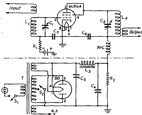
Fig. 1 — Circuit diagram of the doubler stage that is added to the 150-B for 14-Mc. operation.
