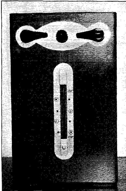
Hydraulic rotator control and direction indicator. The box is 6 x 10 x 11 inches.
