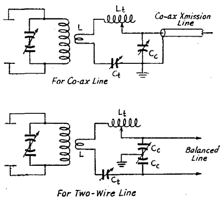
Fig. 4—Harmonic-suppressing circuit for coupling into flat lines. L is the pick-up link, consisting of one or more turns as required. One-turn links may be constructed as shown in Fig. 6 to reduce coupling through stray capacitance. L_t and C_t should be adjusted to resonate the whole circuit, including L and C_c , at the operating frequency. Capacitance values in \mu\text{fd} . for C_c are as follows:
