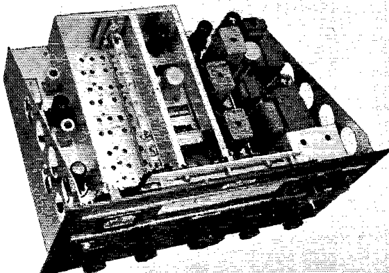
A top view of the Collins receiver with the cover plate removed from the tuning assembly. The many holes are for trimmer adjustments in the r.f. and first i.f. stages — note the movable tuning platform on one side of the compartment.
