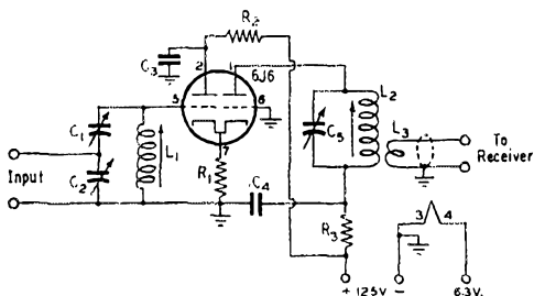
Fig. 3—Circuit diagram of the cathode-coupled preamplifier.
