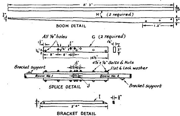
Fig. 4 — Details of the boom, center splice and braces used in the 24-element array.
