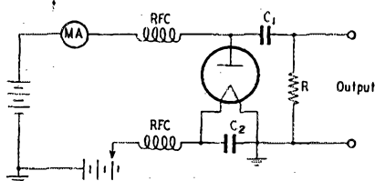
Fig. 1 — The basic circuit of the diode noise generator for measuring receiver sensitivity. By controlling the filament temperature of the diode, the d.c. current through the diode is a direct measure of the noise power developed across R.
