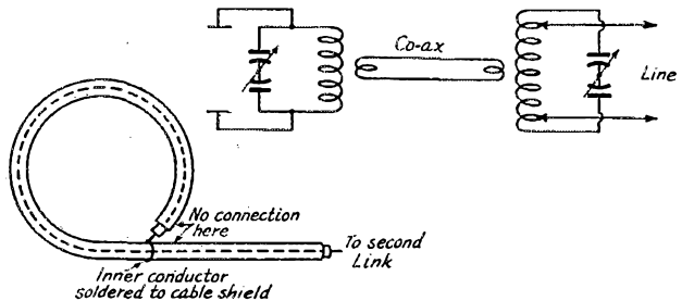
Fig. 6 — Self-shielded link for reducing capacity coupling between inductively-coupled circuits. It is simply a piece of co-ax cable formed into a single turn, with the inner conductor at the end soldered to the outer shield braid as shown. Its application to a link-coupled antenna tuner is shown in the diagram.
