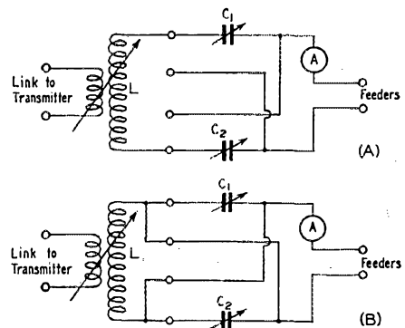
Fig. 5 — Circuit diagram of the antenna coupler for use with the compact medium-power transmitter. A — series tuning. B — parallel tuning.
