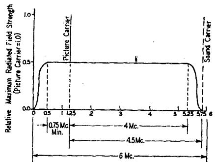
Fig. 1 — The television channel and ideal transmitter frequency characteristic for the picture signal.
