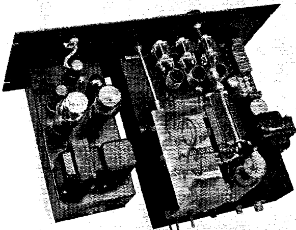
Top view of the speech amplifier-r.f. exciter unit. The speech-amplifier equipment is mounted on the 3 \times 5 \times 10 -inch standard chassis to the left. The r.f. unit is spaced two inches from it with interconnections cabled through a grommetted hole in the side of each chassis. The coil assembly for the plate circuit of the 807 stage is mounted on a bracket bent from sheet aluminum. It is 3\frac{1}{2} inches wide, 6\frac{1}{2} inches long, and 2\frac{1}{2} inches high.
