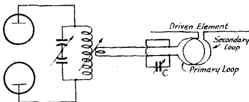
Fig. 1 — Circuit of the coupling system. Primary and secondary loops are identical. C is the tuning condenser. A 400-ohm open line is used.
