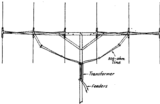
Fig. 1 — Detail drawing of the W2NLY 24-element array.
