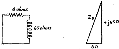
Fig. 2—The secondary circuit and the impedance triangle.
