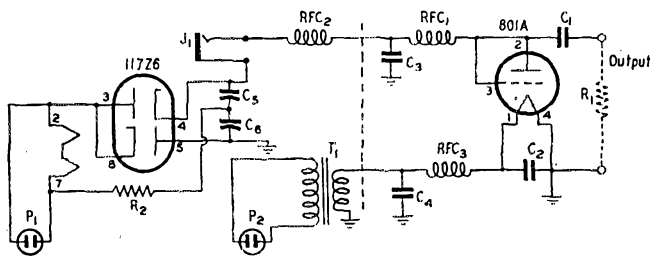
Fig. 2 — A practical circuit for a diode noise generator. The filament temperature is controlled by a Variac or rheostat in series with the a.c. to P 2 .
