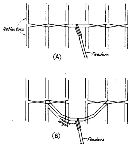
Fig. 2 — The 24-element array was fed originally as shown in A. Unequal current distribution made it necessary to change to the split system shown in B.
