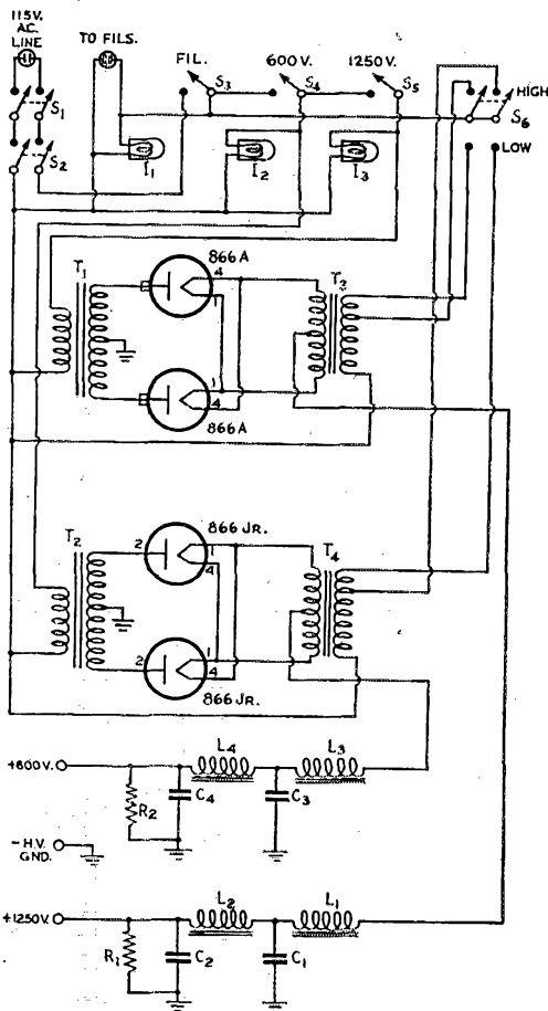
Fig. 4 — Circuit diagram of the dual power supply for the medium-power bandswitching transmitter, delivering 1250 volts at 550 ma. and 600 volts at 200 ma.
