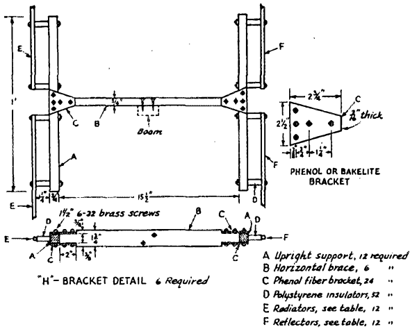
Fig. 5 -- Antenna elements are mounted in six sets of four each (two radiators and two reflectors) on an H-shaped bracket attached to the main boom.
