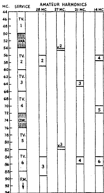
Fig. 3 — The relationship of amateur-band harmonics, 14 to 28 Mc., and frequency assignments in the 44-88 megacycle region.
