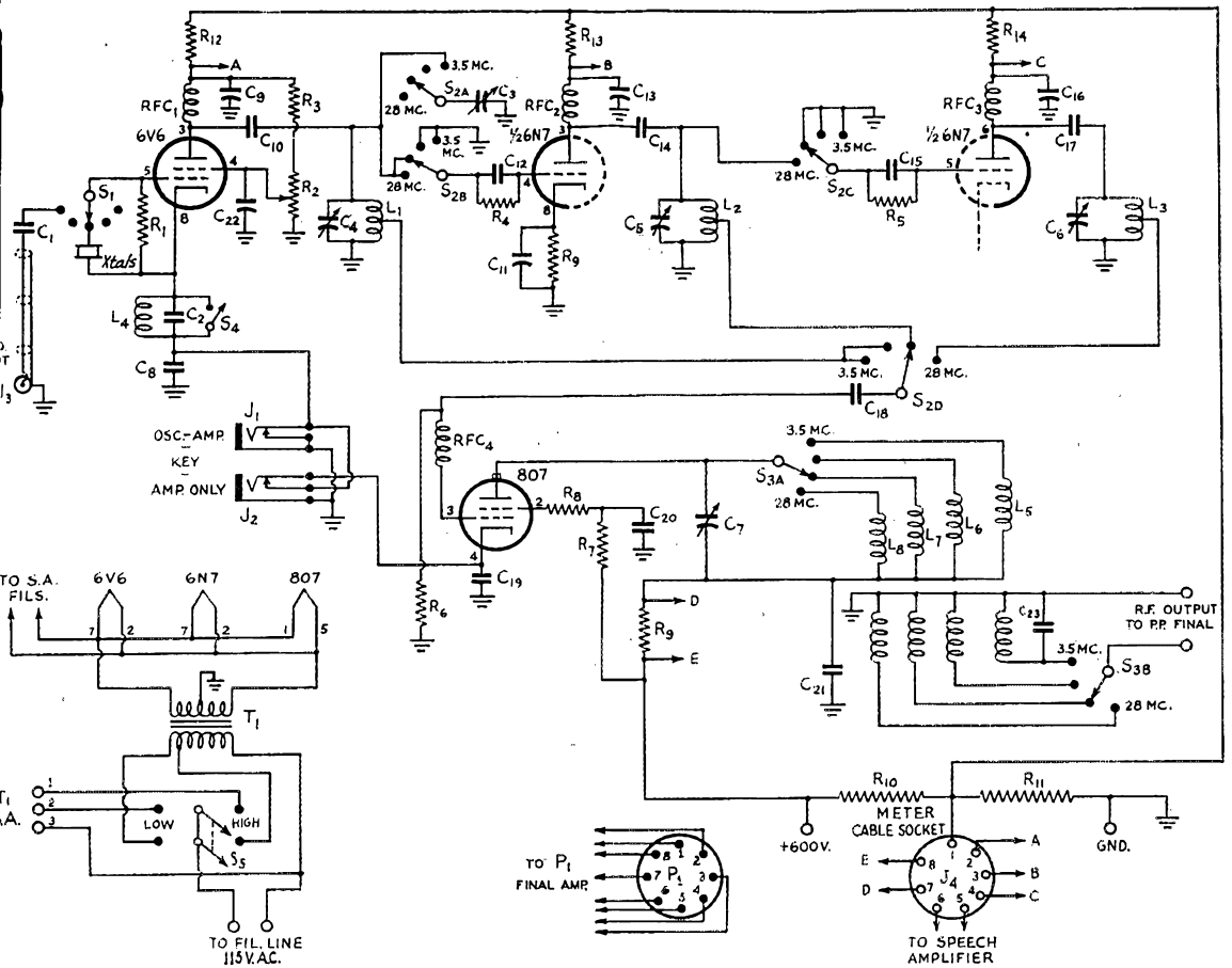
Fig. 1 — Circuit diagram of the r.f. exciter unit.
