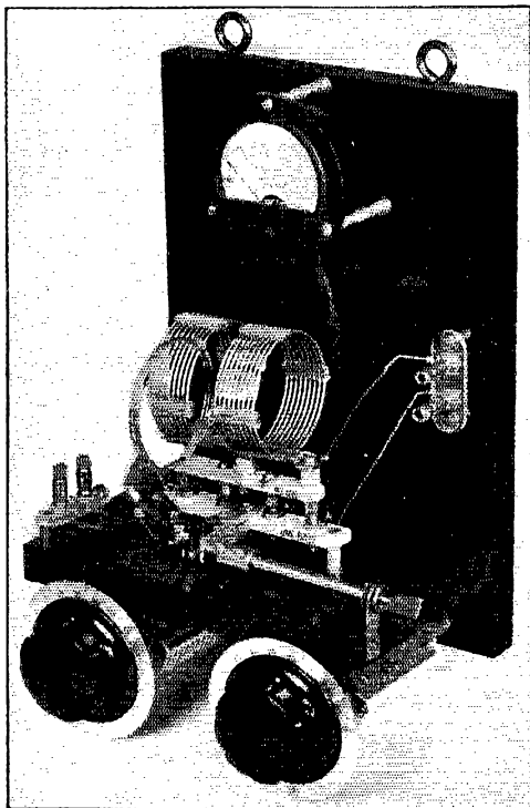
A wall-mounting antenna tuner for the medium-power bandswitching transmitter.
