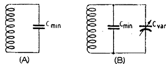
Fig. 1 — A — Circuit for f_{\max} . B — Circuit for f_{\min} . C_{\min} is the total minimum circuit capacitance which includes tube capacitances, minimum capacitance of the tuning condenser and capacitance introduced by sockets and wiring as well as the distributed capacitance of the coil. C_{\text{var}} is the variable part of the tuning-condenser capacitance (maximum minus minimum).
