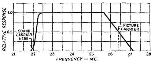
Fig. 2 -- Ideal response curve for the receiver picture i.f. channel, for reception of a signal of the type shown in Fig. 1.
