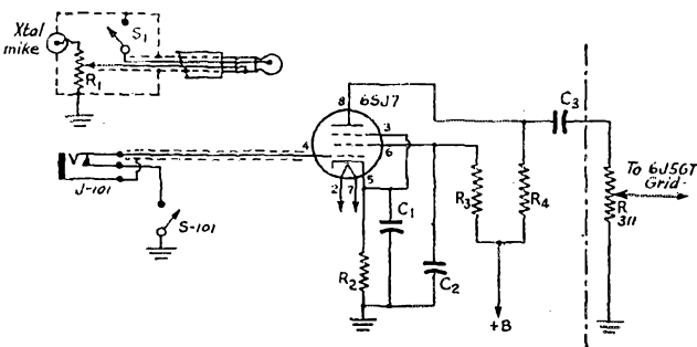
Fig. 2 — Diagram of speech-amplifier stage added to 150-B modulator to permit use of a crystal microphone.
