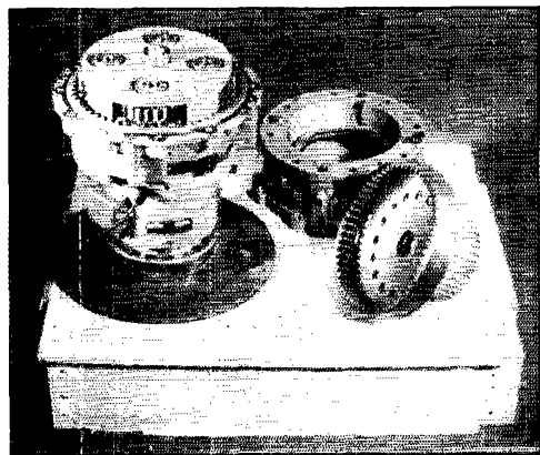
Fig. 1—The "works" inside a propeller-pitch beam rotator. The ring gear mentioned in the text is shown at the right, in front of the upper gear housing. The gear carrier, which is to be drilled and tapped, is still fastened to the top of the assembly. After modification, rotation speeds up to 5 r.p.m. may be obtained with these motors.
