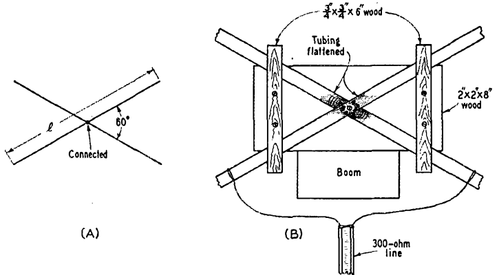
Fig. 2 — The "biconical" beam uses a double element for each element in the usual 3-element beam. Crossed elements as shown at A are used, and the 60-degree angle has been found to give maximum gain. The driven element can be fed with 300-ohm line by tapping it on the elements a little distance each side of center. See text for dimensions.
