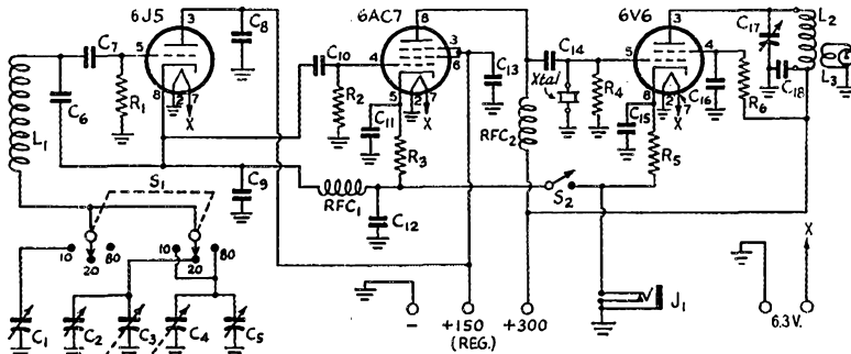
Fig. 2 — Circuit diagram of the 'phone-band VFO.
