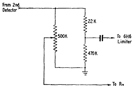
Fig. 3 — A substitute circuit for R_5 of Fig. 2.
