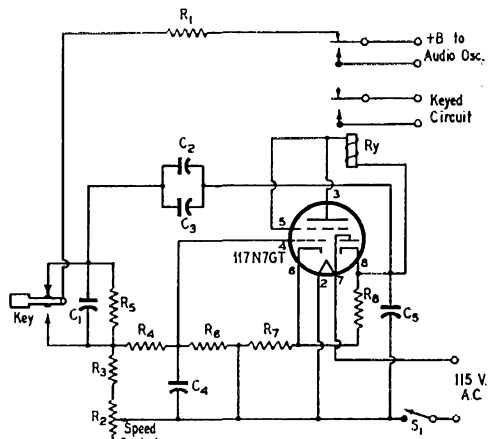
Fig. 4—Circuit diagram of a simplified electronic key.
