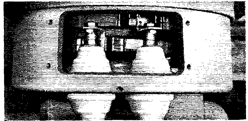
Interior view of rotator showing efficient RF slip rings.
