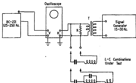
Fig. 7 — The method used for checking coil-and-condenser combinations. An accurate frequency check is obtained by using a BC-221 to check the 10th harmonic of the test signal generator. The LC combination under test is adjusted for minimum horizontal amplitude at the desired frequency.
