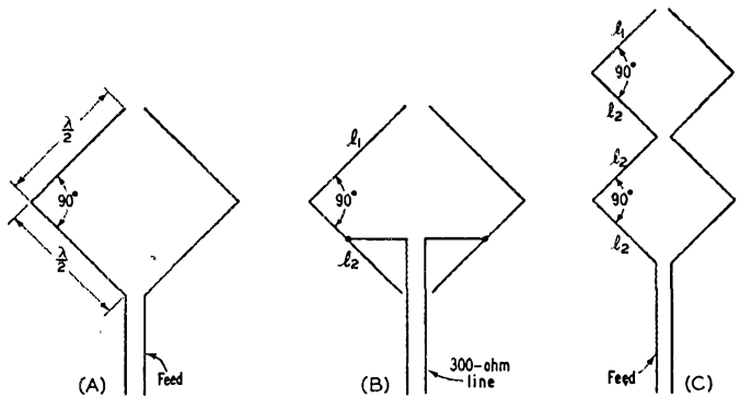
Fig. 1 — The 90-degree inverted rhombic at A is better known to amateurs as the "bisquare" antenna. It can be fed without special matching sections by tapping the feeders on to the elements, as shown in B (see text for dimensions). How several sections can be stacked and fed at the bottom is shown at C.
