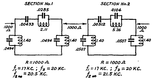
Fig. 3 — Component values of the individual pi sections of the filter. Values are in \mu fd. and mh.
