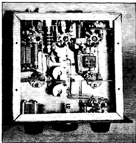
Bottom of the chassis in the 'phone-band model VFO. The three air trimmers are at the center. The condenser in the lower left-hand corner is the doubler tank condenser. The handsread switch is to the right.
