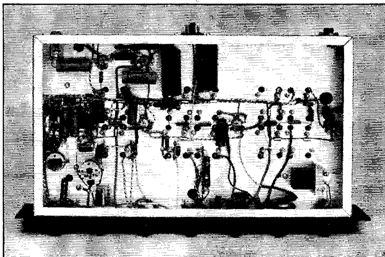
◆ Underneath the chassis of the 50-kc. amplifier. ◆
