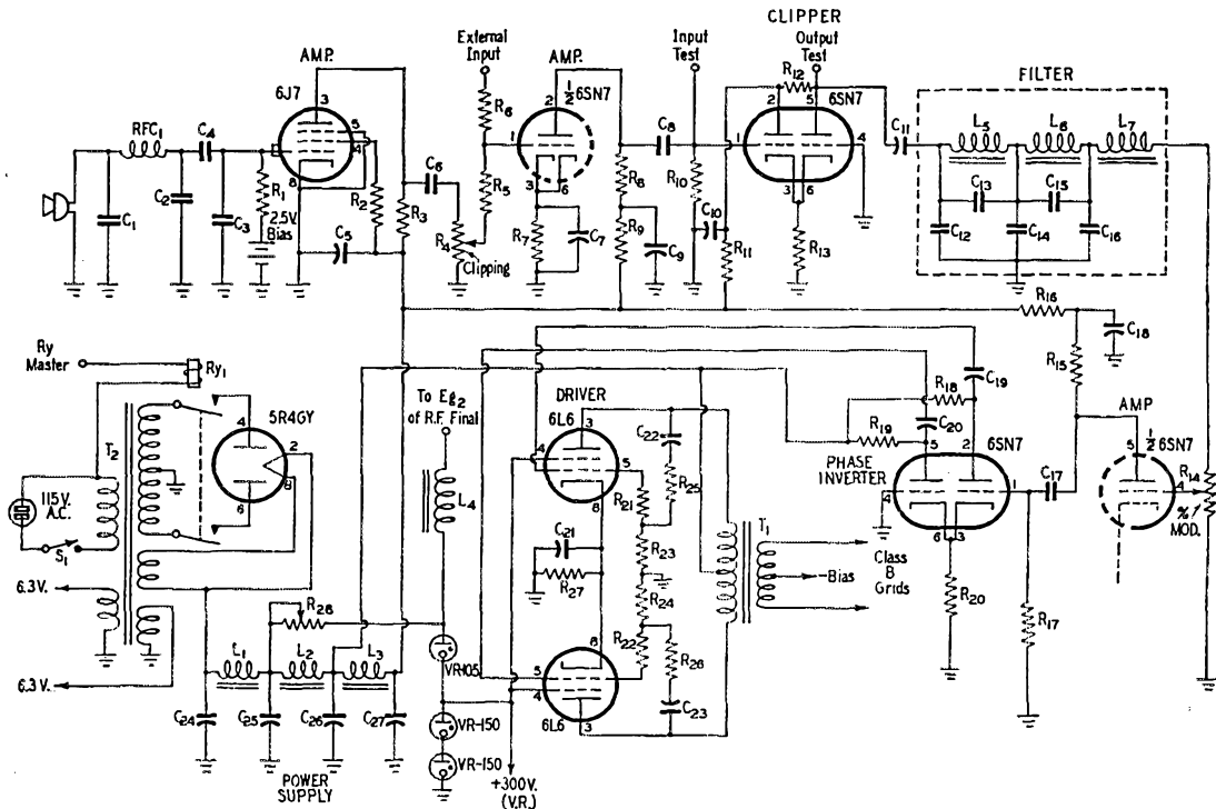
Fig. 1 — Circuit diagram of the clipper-filter speech amplifier.
