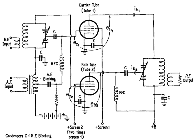
Fig. 4 — The basic circuit of the "supermodulation" system as interpreted by W6QYT.
