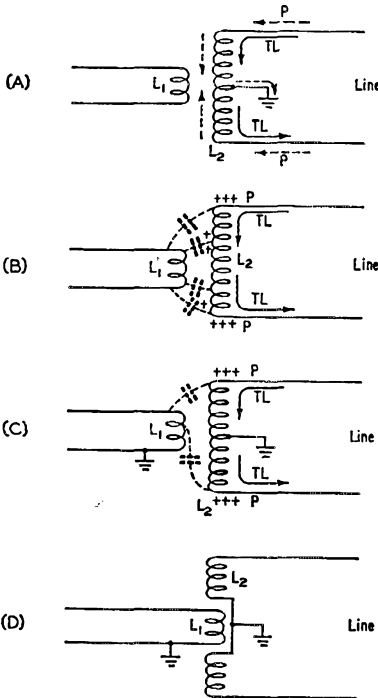
Fig. 3 — By using a balanced circuit and taking precautions to reduce capacitive coupling between the coils, the effects of parallel currents on a two-wire line can be made negligible in the measuring circuit.
