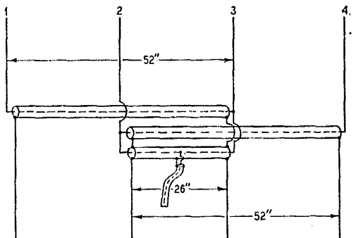
Fig. 1 — Driven element arrangement used by W5KFY. A director and a reflector are used with each of these, to make a 12-element array.
