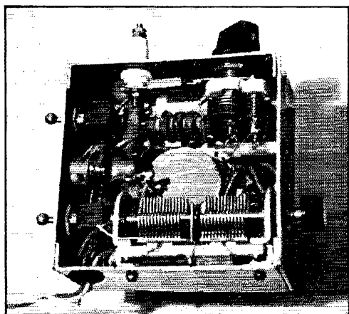
Bottom view of the secondary frequency standard.
