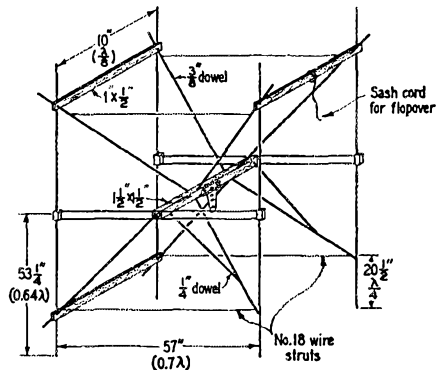
Fig. 1 — Detail drawing of the lightweight flopover array described by W2WFB.
