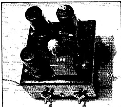
A simple 100-kc. frequency standard giving 10-kc. points.
