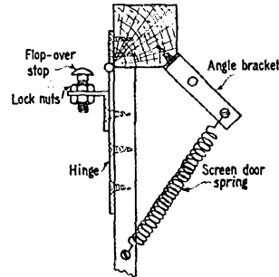
Fig. 3 — Details of the floppover arrangement.
