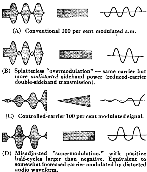
Fig. 1 — Amplitude-modulation waveforms.
