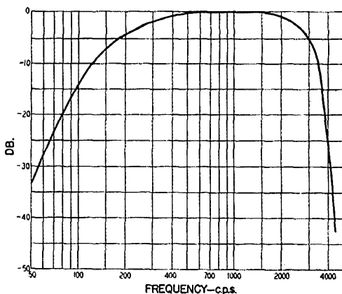
Fig. 2 — Frequency response curve of the amplifier of Fig. 1.
