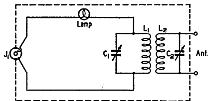
Fig. 2 — Harmonic separator for the antenna.
