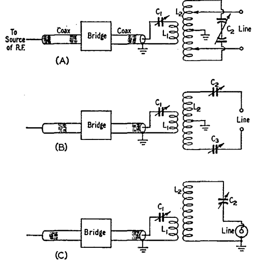
Fig. 4 — Recommended practical circuits. An antenna coupler with a fixed link can be used at A, and C_1 may be left out if the link is large enough to couple properly. Practical considerations in using the other two circuits are discussed in the text.
