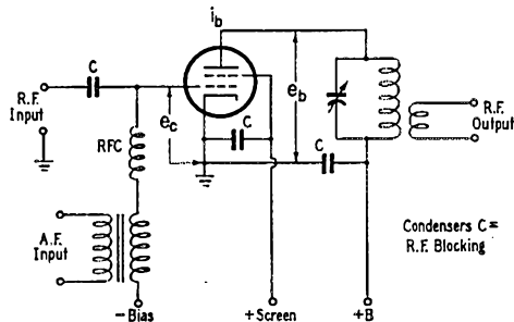
Fig. 2 — Basic circuit, ordinary grid-bias modulated amplifier.
