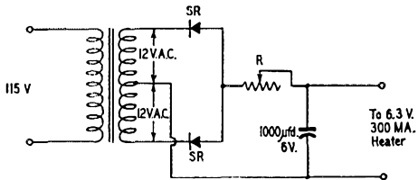
Fig. 1 — Circuit diagram of a d.c. heater supply for hum reduction in oscillators, speech amplifiers, etc.
