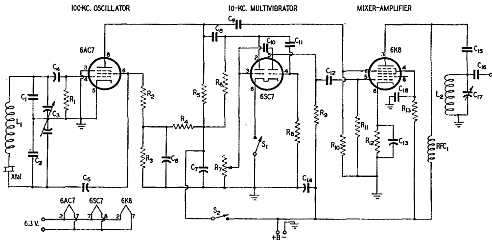
Fig. 1 — Circuit of the secondary frequency standard.
