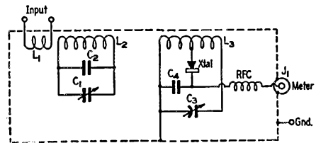
Fig. 1 — Harmonic checker for use in supply leads.
