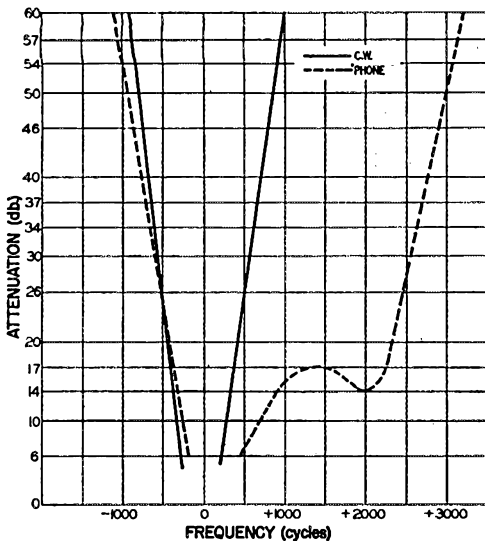
Fig. 4 — Measured selectivity of the i.f. amplifier, as used for c.w. and for 'phone reception.
