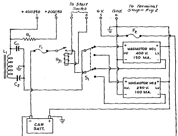
Fig. 3 — Wiring of the power-supply unit.
