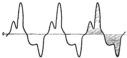
Fig. 1— This and any other periodic wave can be resolved into a fundamental and series of harmonically-related sine waves. The axis of the wave is at the point where the total areas above and below are equal — i.e., the average positive amplitude is equal to the average negative amplitude and the algebraic sum is zero.
