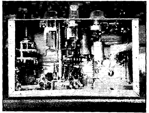
Bottom view of the all-band 'phone-c.w. mobile transmitter.
