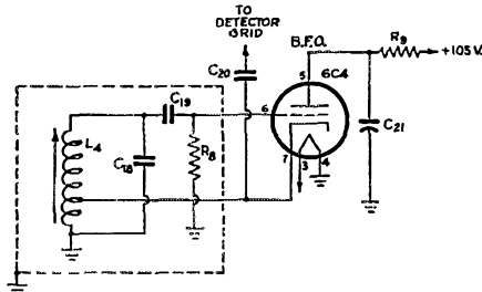
Fig. 3 — Circuit of the superhet b.f.o.
