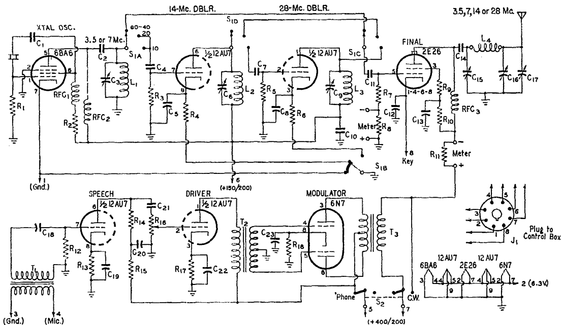
Fig. 1 — Circuit diagram of the all-hand transmitter.
