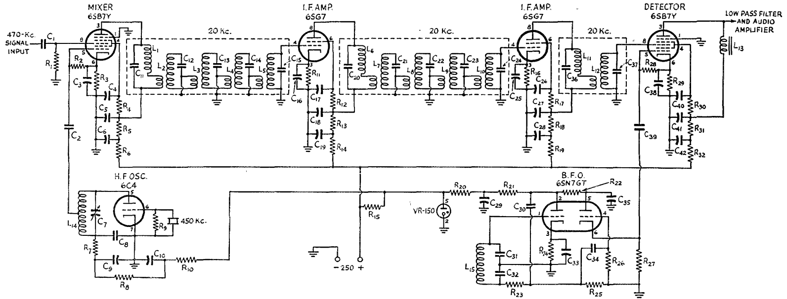
Fig. 1 — Wiring diagram of the 20-kc. i.f. amplifier.
