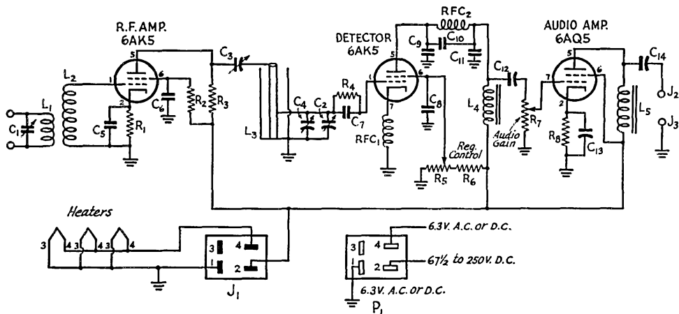
Fig. 1—Schematic diagram and parts list for the Novice-Technician v.h.f. receiver.
