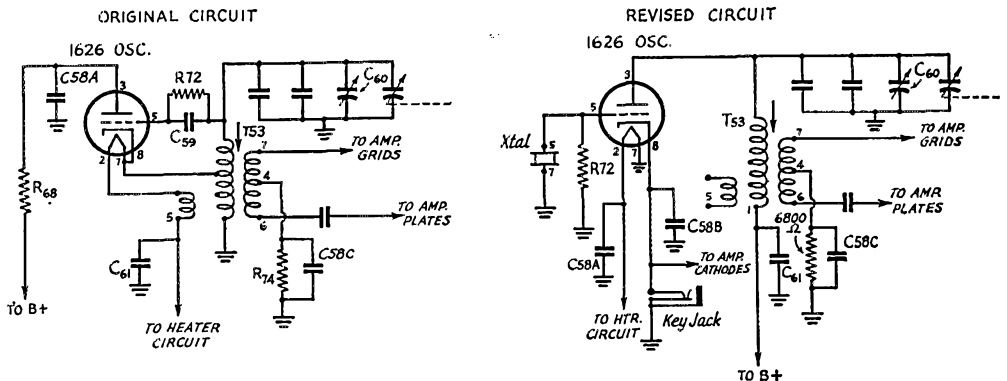
Fig. 1— "Before" and "after" versions of the oscillator circuit. Note that the principal change is the transfer of the tuned circuit from the grid to the plate. A crystal is used in the grid circuit. The diagram has been simplified by the omission of the calibrating circuit, which is removed from the transmitter. Symbol designations are those used in the diagrams of the original equipment, and are used here for reference purposes only. Values, where different from the original, are given in the text.
