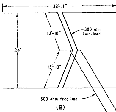
Fig. 2—The two antenna systems that were tested by W3KQU. That at A is simply a 14-Mc. half-wavelength antenna with a two-band feed, and that at B is two 14-Mc. halfwave antennas with \frac{3}{8} -wavelength spacing, fed in phase.
