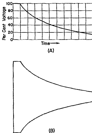
Fig. 3 — (A) Behavior of d.c. plate voltage on Class C amplifier when the plate-supply voltage is suddenly reduced to zero. (B) Corresponding oscilloscope pattern of r.f. envelope.
