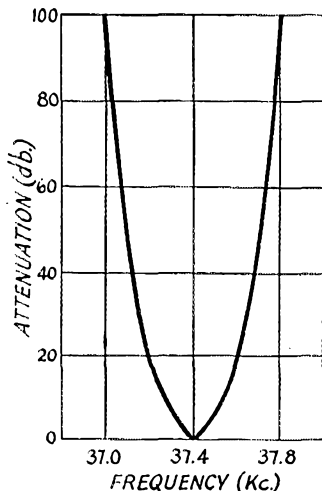
Fig. 2 — Selectivity characteristic of the 37-kc. i.f. amplifier.
