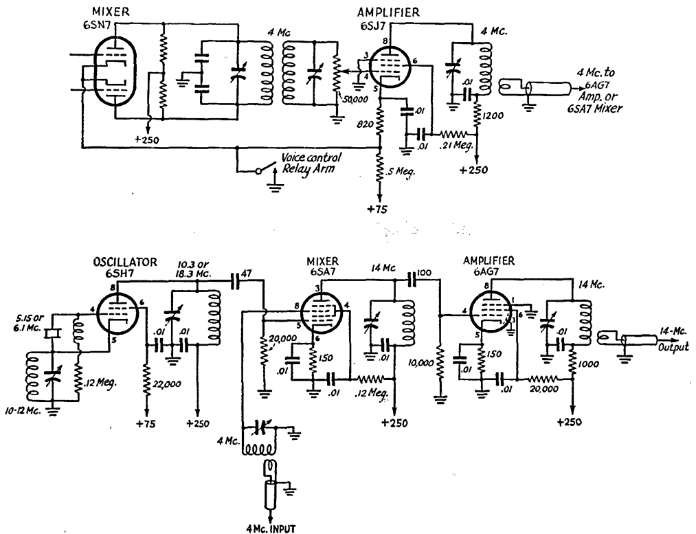
Fig. 1— Here is the way W2FGV converts the 4-Mc. output from his Edmonds (W1JEO) exciter to 14 Mc. The top circuit shows the only modification in the original circuit, the addition of the 6SJ7 amplifier, and the bottom circuit shows the 6SA7 mixer and a 6AG7 amplifier working on 20. John has the whole thing built on a 13 × 17 × 3-inch chassis and uses it to drive a pair of 807s running 125 watts on either 75 or 20.
