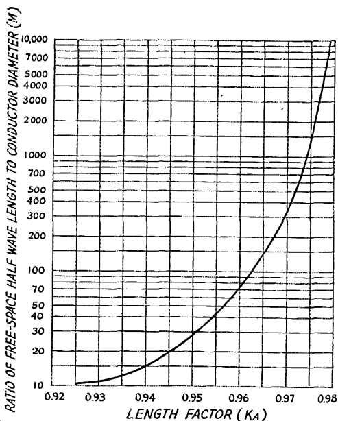
Fig. 2—The antenna-length factor as a function of the ratio of a free-space half wavelength to the conductor diameter. The length factor multiplied by a free-space quarter wavelength is the length of a quarter-wave radiator resonant at the selected frequency.
