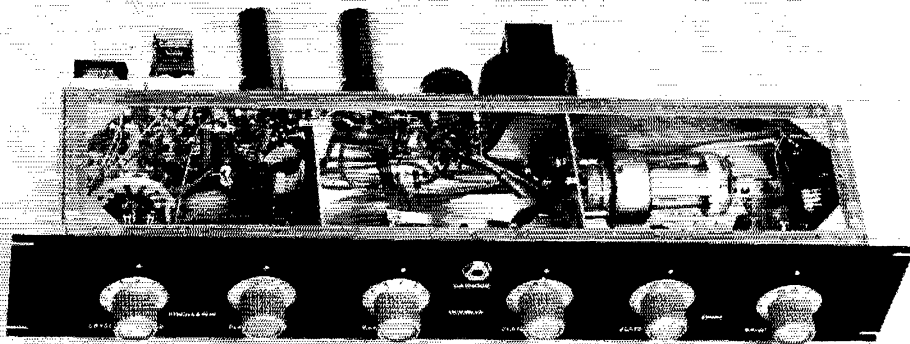
Looking into the handswitching exciter-transmitter from the top front. Oscillator components are in the left compartment, the doubler and power connector in the center, and the output stage at the right. Note that the 6146 socket is mounted inside the output stage compartment.
