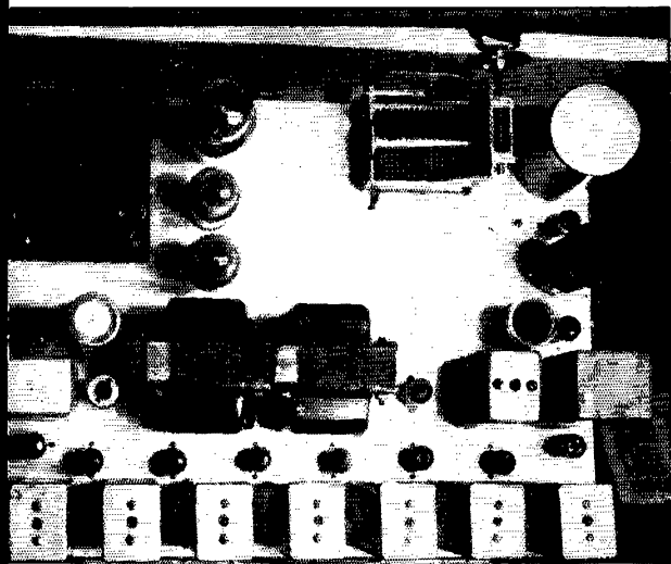
A top view of the receiver shows the precision tuning condenser used for tuning (top right) and the string of 37-kc. tuned circuits (bottom).
