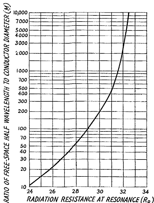
Fig. 4—Radiation resistance of a quarter-wave antenna (with ground plane or grounded) as a function of M . The values apply only when the antenna is of the resonant length. Multiply resistance values by 2 for half-wave antennas.
