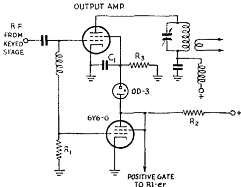
Fig. 3—The positive gate for the “R1-cr” can be obtained from the plate of the conventional clamp tube, as shown here. C_1 — 0.005 \mu\text{fd.} R_1 — Normal grid leak. R_2 — Normal screen-dropping resistor. R_3 — 0.47 megohm.
