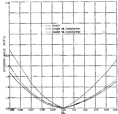
Fig. 4 — A special case showing a 65-ohm antenna matched by a 65-ohm transmission line (solid curve) and to a 500-ohm line through single and double "Q" transformers. (Data from Kraus, Antennas , McGraw-Hill Book Co., N. Y.)
