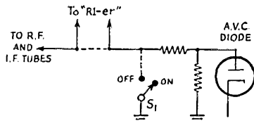
Fig. 4—Receiver changes necessary to add the “R1-cr” are shown by the dotted lines. The a.v.c. switch, S_1 , is disconnected (or left open if it is a single-function switch), and the a.v.c. line is broken and connected to the points shown in Fig. 2.
