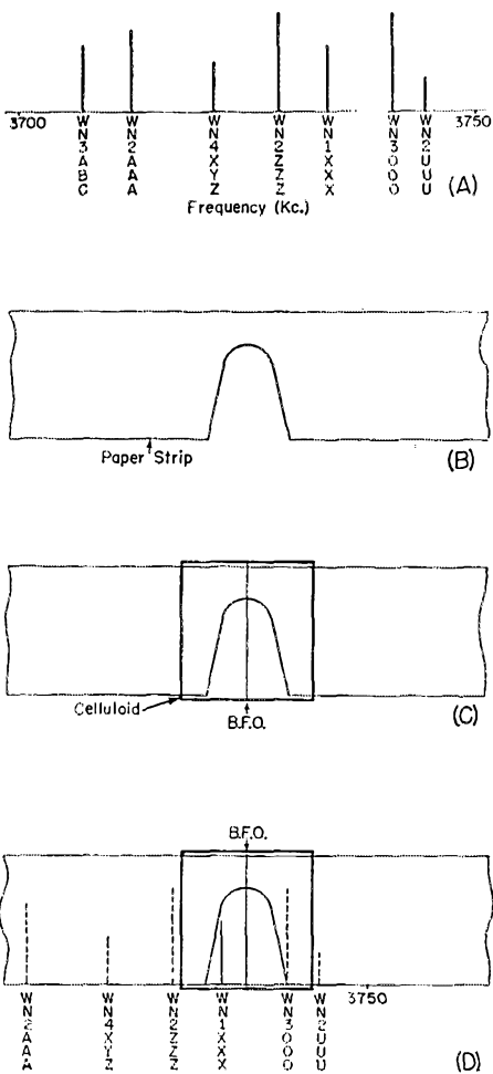
Fig. 1 — An illustration of some of the principles of receiver operation. At some given time, the 80-meter Novice band might look like A, the vertical lines corresponding to the signals of the calls given below.
