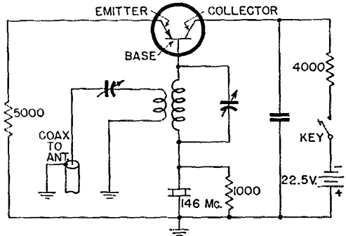
Fig. 1 — Schematic diagram of the transistor crystal oscillator used on 146 Mc. by K2AH. The only unfamiliar element is the symbol for the transistor itself. Values in the tuned circuits are dependent on the frequency used, but this general circuit works with crystals of much lower frequency as well.
