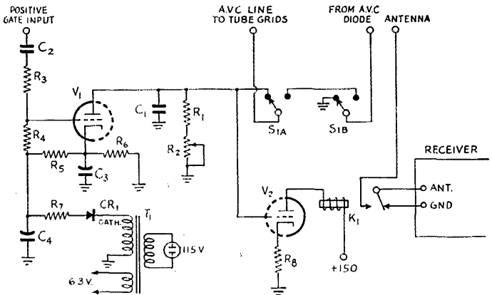
Fig. 2 — The practical TVG circuit.
