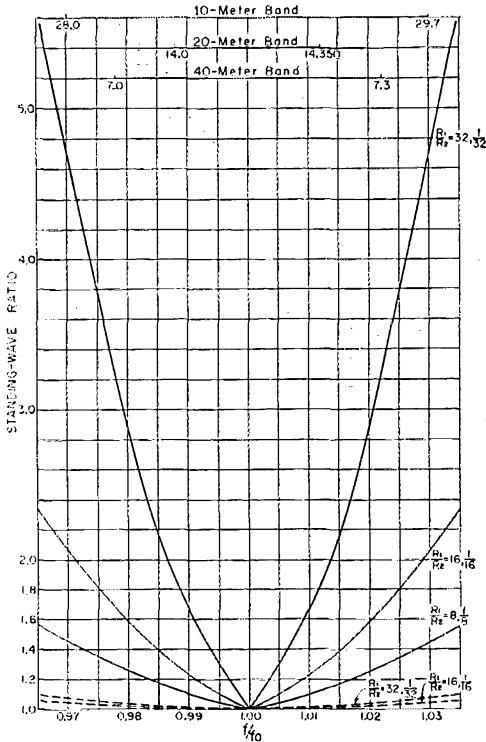
Fig. 2 — Effect of "Q"-section on selectivity, as expressed by the s.w.r. on the line to which the antenna is matched at the desired frequency, f_0 . As shown, the selectivity depends critically on the ratio of the two impedances to be matched. These curves do not include the selectivity of the antenna itself.
