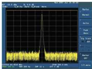
3kHz filter characteristics (500kHz span)
