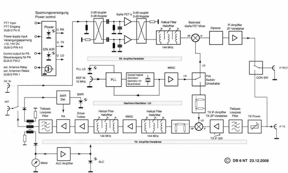
TR 144 H +40 Transverter Blockdiagramm/block diagram
