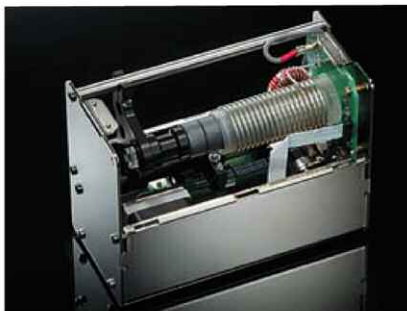
● RF μ-Tuning Unit Photo
