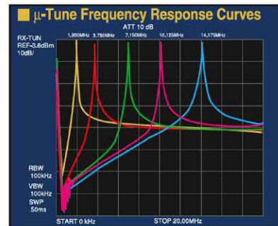
10 dB/Div · 2 MHz/Div
