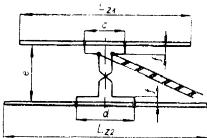
Obr. 108. HB9CV-beam
