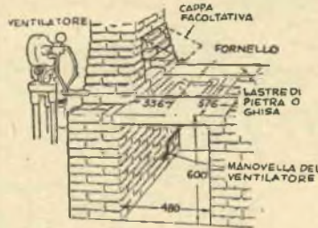
FORGIA IN MURATURA
