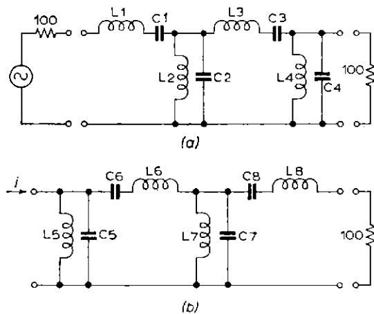
Fig. 13 — Input (a) and output (b) filters for use with the wide-band amplifier
