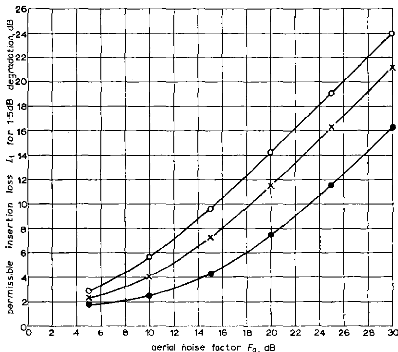
Fig. 1 — Permissible insertion loss L_1 between aerial and receiver for a degradation of 1.5 dB
