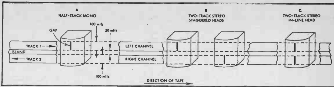
Figure 1: Head configurations for half-track mono, and two forms of two-track stereo. The in-line head arrangement, as at "C," is now the recognised standard and corresponds with the in-line heads used on four-track machines.
