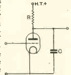
Fig. 1.—Circuit possessing high-note cut-off.
