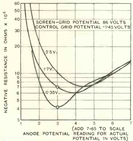
Fig. 16.—Negative resistance curves for various amplitudes associated with the oscillation conditions of range 4 of the dynatron wavemeter.
