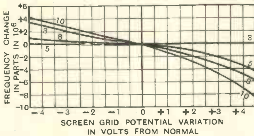
Fig. 13.—Curves showing the observed change of frequency of Sullivan-Griffiths dynatron oscillating wavemeter due to variations in screen-grid potential. The permissible potential fluctuation is \pm 1 volt and the greatest inaccuracy introduced by this 1 part in 10^6 (at the lower frequencies).
