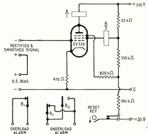
Fig. 6. Amplifier speech-level alarm.
