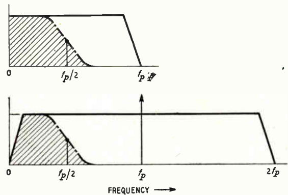
Fig. 14. The spectrum of the signal S when transmitted by a dot-interlace system for a single signal. - - - - = amplitude characteristic of the transmission filter.
