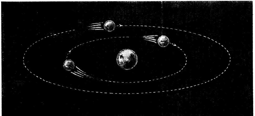
Fig. 9. Diagram of a lithium atom, with a trebly charged nucleus, and with an extra electron revolving outside the group seen in the helium atom, conferring on the atom (lithium) strong chemical properties
