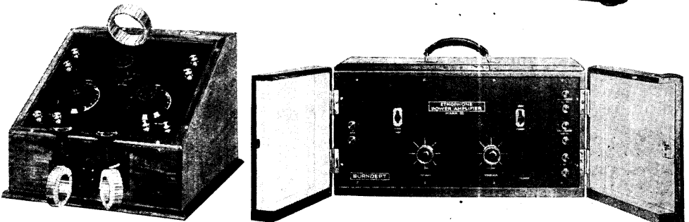
Fig. 5 (left). This is the Home Constructor's set No. 3, which may be built by the amateur. Fig. 6 (right). Made specially portable is an Ethophone power amplifier. Two L.S.2 valves are used
