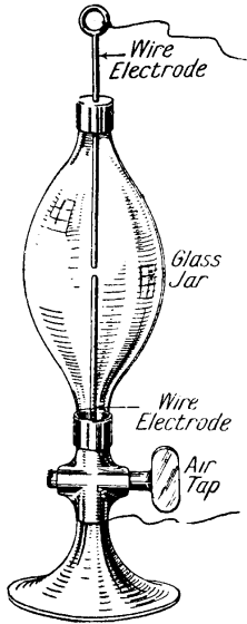
Fig. 1. Faraday's apparatus for demonstrating his "dark space." It consists of a glass jar containing two adjustable rods in a partial vacuum. An electric discharge between the rods included a "short dark space"
