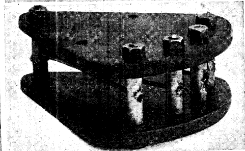
Fig. 1. Spaced apart are two pear-shaped plates. The broad end holds the aerial leads, and the bottom a common lead to the instrument. Fig. 2. Details of one of the side plates of the fan antenna connector. The material is ebonite \frac{1}{4} in. thick, cut to shape and drilled to dimensions given. Fig. 3. Both plates are drilled together to ensure accuracy of fit for the spacers. The ebonite plates are held in a vice and pierced with a hand drill, as illustrated. Fig. 4. Cross-bars and spacers are shown fitted to one side of the connector. Fig. 5. Connexions are made from the cross-bars to the lead-in connector by metal bars. These are soldered. Fig. 6. Cross-bars are held by nuts. This view shows the fan antenna connector complete
