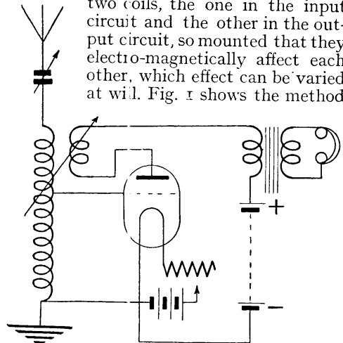
PLATE AND GRID OF FEED-BACK CIRCUIT
