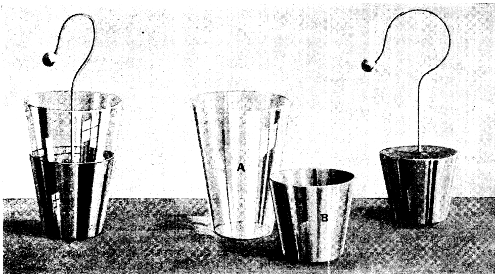
Fig. 2. This apparatus emphasizes the importance of the dielectric. A, B, and C, being packed together as shown on the left, can be charged as a Leyden jar. With an insulating handle they can then be taken apart, separately as A, B, and C, being then apparently discharged. But when the parts are put together again, a strong spark can still be got between B and C, showing that the charge really resided on the glass, A, the coatings merely acting as conductors
