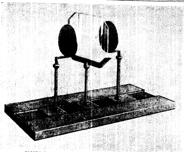
SIMPLE FORM OF VARIABLE CONDENSER
