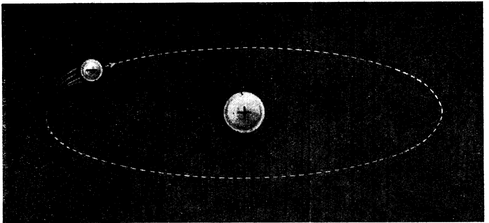
Fig. 7. Diagrammatic representation of the normal hydrogen atom, the simplest of all the atoms. It consists of a negative electron revolving round a positive nucleus. Its orbit is dotted
