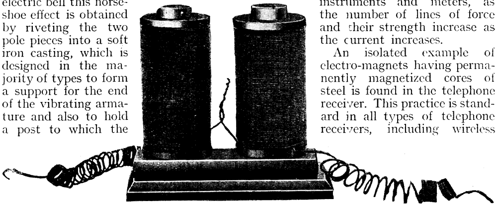
ELECTRO-MAGNETS SUITABLE FOR A MORSE INKER
