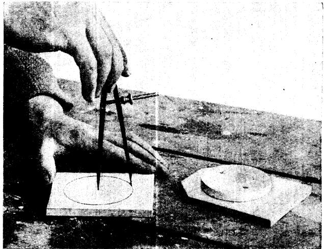
PREPARING END CHEEKS FOR A COIL
