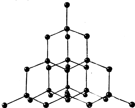
Fig. 16. Model of racemic acid, showing eight molecules, four of which would rotate the plane of vibration of light waves in one sense and four in the opposite sense
