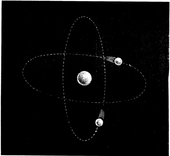
ELECTRONS IN THE ATOM OF HELIUM
