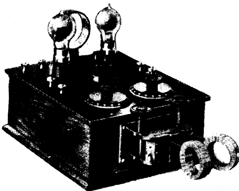
"POPULAR" ETHOPHONE
