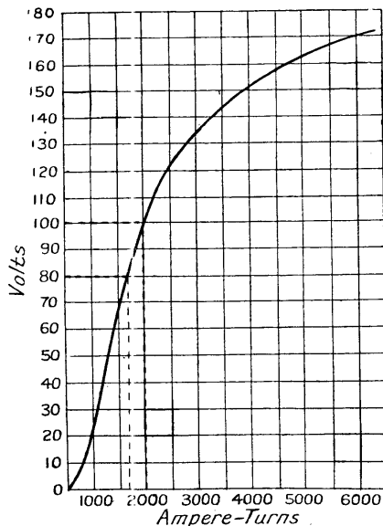
SATURATION CURVE OF A DYNAMO
