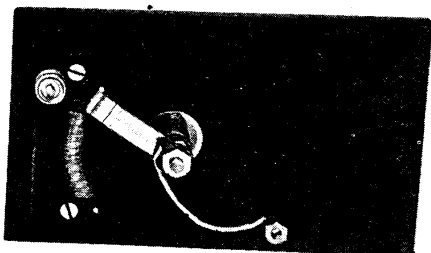
Fig. 7. Details of the back of the panel of an easily made rheostat, showing contact arm
