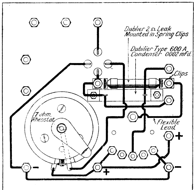
Fig. 10. The position of all the wiring is shown approximately in this diagram of the rear of the experimenter's panel. Comparison can be made with the front diagram (Fig. 5). Wiring is shown in thick lines. Note the position of the grid leak, and the shortness of connexions
