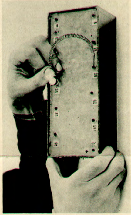
Fig. 2. Continuity of contact in a loose coupler primary is tested with a flashlight bulb. A break in the wiring or imperfect contact is shown by the lamp going out
