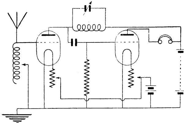
Fig. 15. Correct wiring of a grid leak in a two-valve circuit is shown. Tuned anode and resistance-coupled high-frequency amplification are included in the circuit. It sometimes occurs that the grid leak is shunted across the grid condenser, but in this type of circuit such an arrangement is wrong, and the circuit as shown is correct
