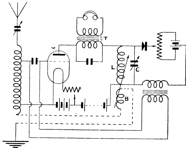
HIGH- AND LOW-FREQUENCY FEED-BACK CIRCUIT
