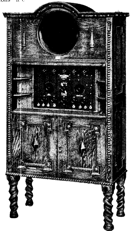
FELLOPHONE SUPER-FIVE SET
