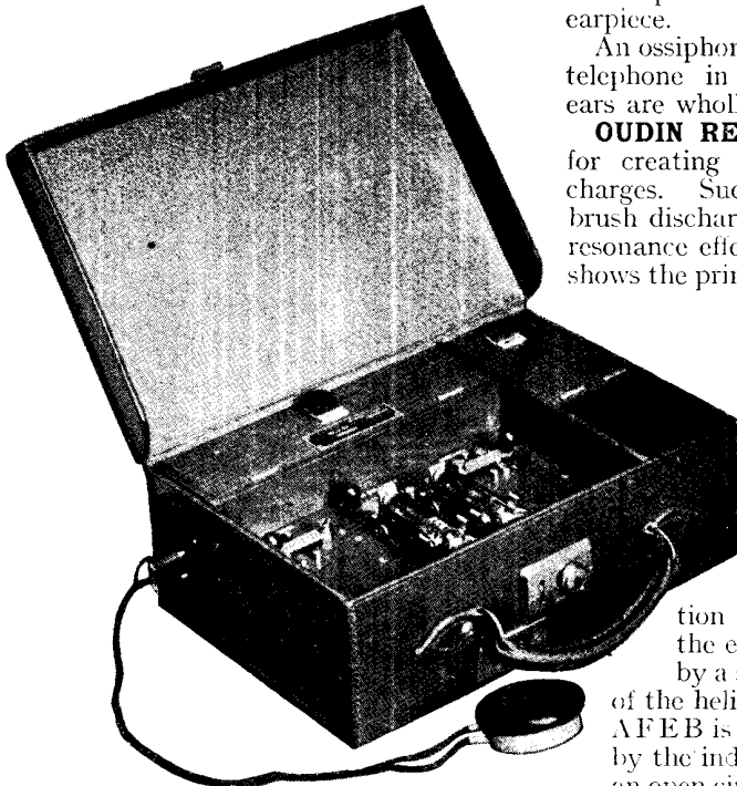
MARCONI OTOPHONE
