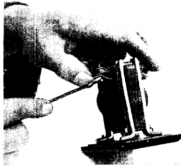
Fig. 21. How the wire is fitted in the spring-clip terminals of this type of low-frequency transformer is seen in this photograph
