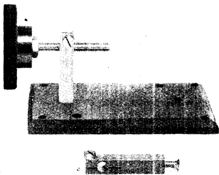
Fig. 7. One post is shown fixed to the base, the other detached, to reveal the slot and clamping screw
