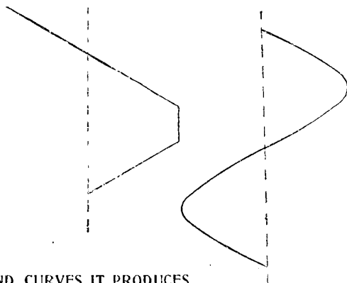
Fig. 1 (left). F is a field coil, W W are stretched wires, G is a guide for the wires, M a mirror, and T is a spring screw for adjusting the tension on the wires; B B are terminals. Fig. 2 (centre). Diagonal and straight paths traced by a beam of light falling on a moving photographic plate. Fig. 3 (right). This is the kind of curve which an oscillograph traces for alternating currents
