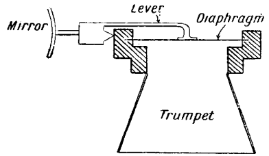
PHOTOPHONE MIRROR AND DIAPHRAGM
