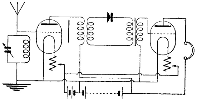
WIRING DIAGRAM OF PORTABLE SET
