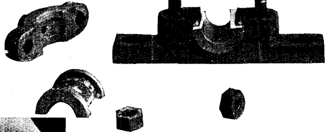
Fig. 7. Very thin packing slips of sheet metal known as shims are used to pack up the inner faces of the two halves of a plummer block
