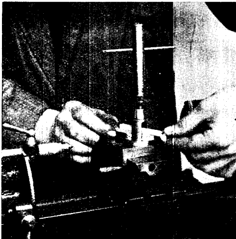
Fig. 6. Beneath a lathe tool metallic or wooden packing is placed. Packing is required to raise the tool to the proper height equivalent to that of the lathe centres
