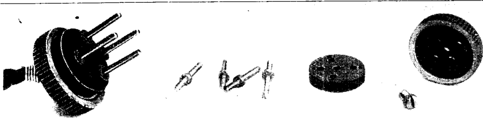
Fig. 5. Connexions for H.T. Fig. 6. Components of the four-pin plug are shown dissembled. and L.T. batteries can be Four valve legs are used as pins, and the ebonite disks are screwed together made by this plug.
