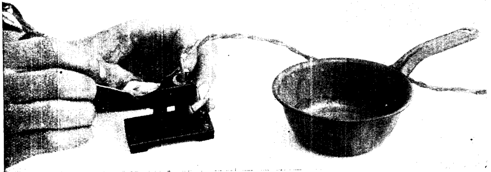
Fig. 11. Complete and perfect insulation is ensured by filling up the recess occupied by the wire and socket base with molten hard wax. The wax is best introduced with the aid of a spoon, care being taken to break any air bubbles in order that the aperture may be completely filled
