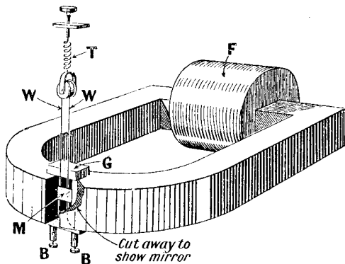
Fig. 1 (left). F is a field coil, W W are stretched wires, G is a guide for the wires, M a mirror, and T is a spring screw for adjusting the tension on the wires; B B are terminals. Fig. 2 (centre). Diagonal and straight paths traced by a beam of light falling on a moving photographic plate. Fig. 3 (right). This is the kind of curve which an oscillograph traces for alternating currents
