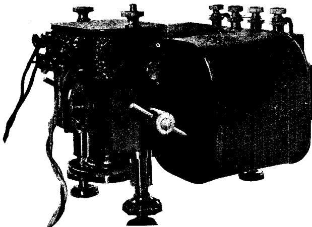
Fig. 7. This is another view of the electro-magnetic control of the oscillograph
