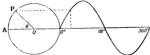
MEANING OF PHASE ANGLE
