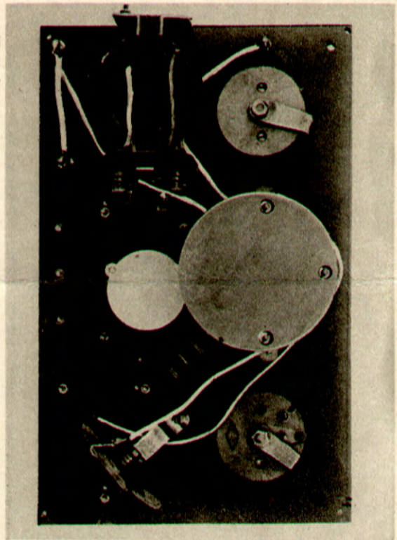
Fig. 6.—Between the two filament resistances the variable condenser is fitted; this is attached by a special top plate with lugs
