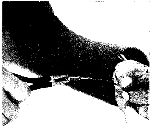
Fig. 7. Across the end of the socket a saw cut is made to enable it to be screwed into the base
