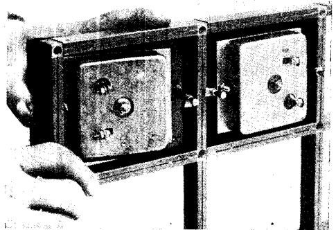
Fig. 10. One condenser panel is clamped in position on the frame, and a second is being fixed in position on the left
