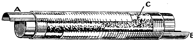
CONSTRUCTION OF A POPOFF COHERER
