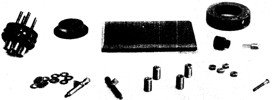
Fig. 17. From this photograph will be seen the simplicity of construction of the Holderstat. The filament resistance is shown on the left, and the actuating plunger and knob are shown on the right
