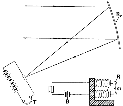
PHOTOPHONE REFLECTOR AND MICROPHONE
