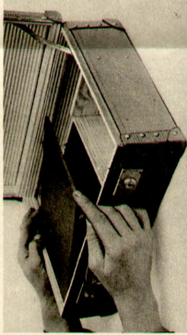
Fig. 4.—Ebonite sheet is cut and trimmed to the dimensions of the compartment to hold the panel
