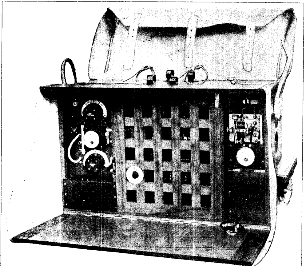
Fig. 21. With the side of the cabinet folded down the transmitter of the portable pack set is seen. The side forms a convenient table for taking down messages
