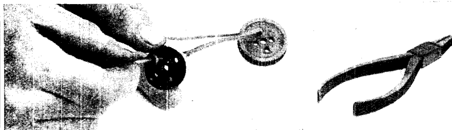
Fig. 7. This photograph shows the assembling of the first wire. Note how the wire is threaded through both disks. The assembly must be done very carefully to ensure sound contacts
