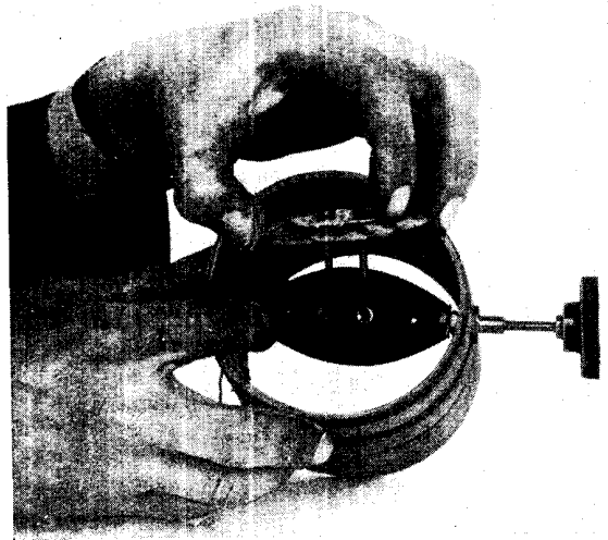
Fig. 10. Another use for a plug-in contact is for adding a reaction coil to a special holder in the interior of the tuning inductance as illustrated
