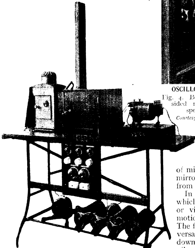
Fig. 5. In the centre is the cupboard containing the electric motor; on the left is the lantern projector
