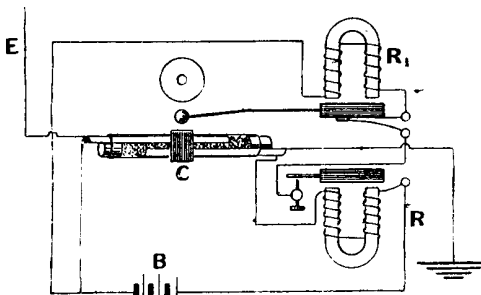
POPOFF COHERER CIRCUIT
