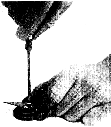
Fig. 1. Screwed to an ordinary turning knob is a simple pointer made of a triangular piece of brass
