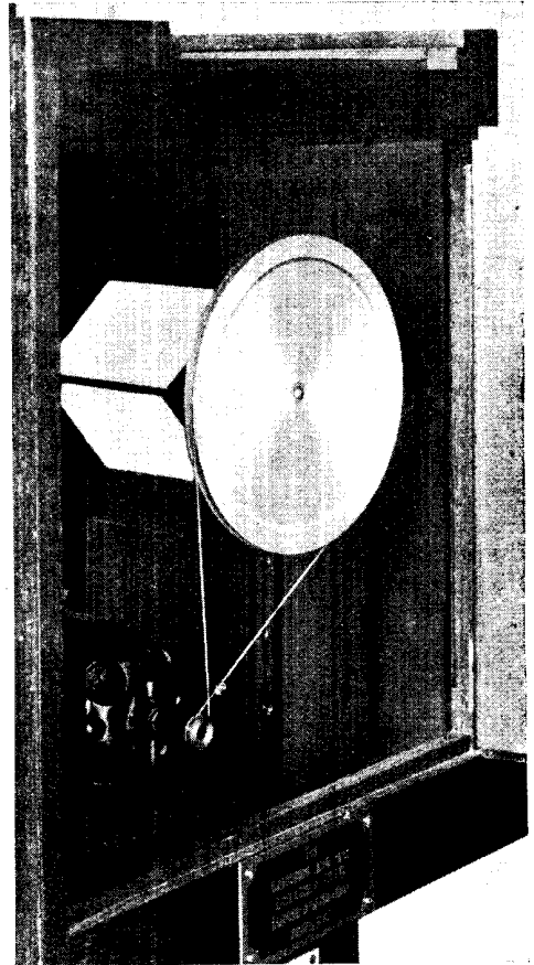
Fig. 4. Behind the rotating disk is a four-sided mirror. This is rotated at a slow speed as compared with the motor
