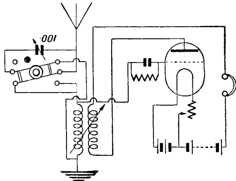
POLAR BLOK ONE-VALVE CIRCUIT
