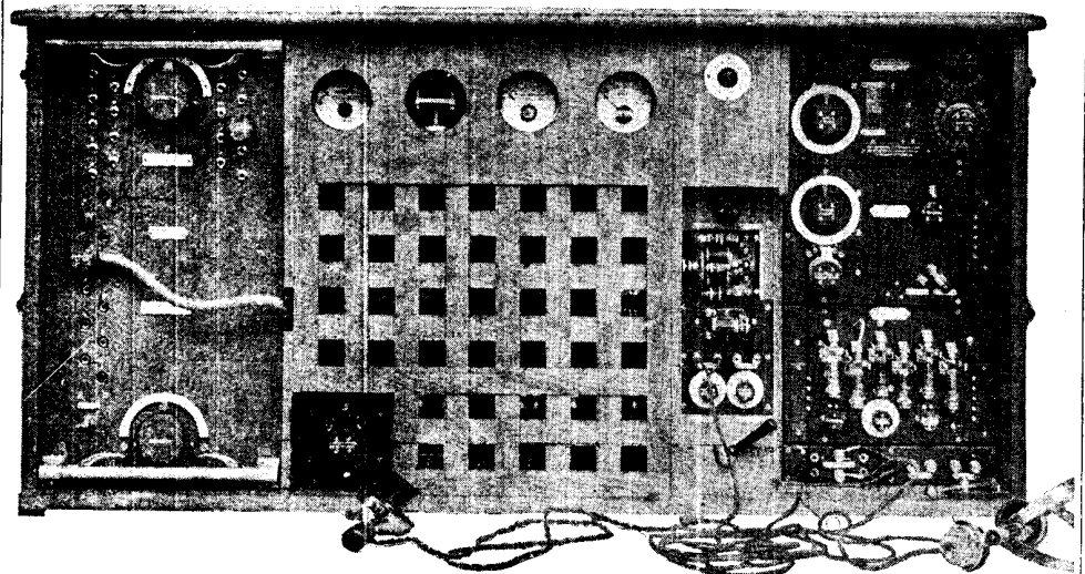
Fig. 22. Marconi's portable set in this photograph is known as type YC2. This is a combined transmitter and receiver housed in one cabinet. The transmitting gear is behind the trellis screen Courtesy Marconi's Wireless Telegraph Co. Ltd.
