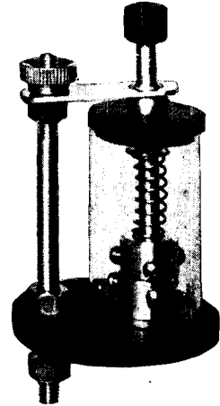
Fig. 5. Vertical type of perikon detector. The pressure between the two crystals is adjusted by a spring
