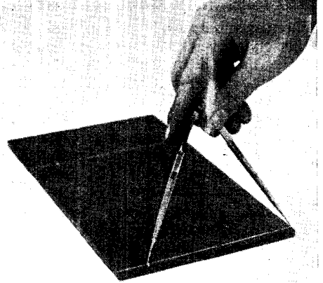
Fig. 2. Mark off equal distances along two reference lines which have been scribed on the panel to ensure cutting square
