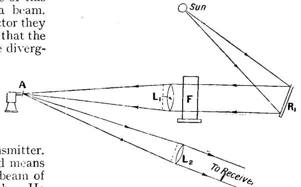
SENDING SOUND BY SUNBEAMS
