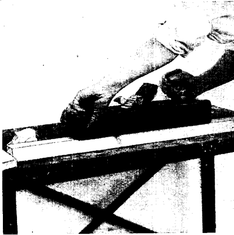
Fig. 4. Both hands are used for planing with a jack plane. The left hand holds the fore part of the body
