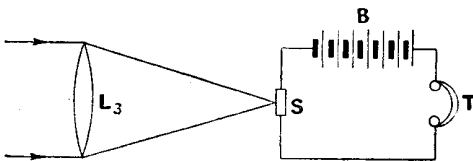
PHOTOPHONE RECEIVER
