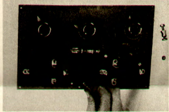
Fig. 7.—On the panel front a neat and efficient crystal detector is fitted
