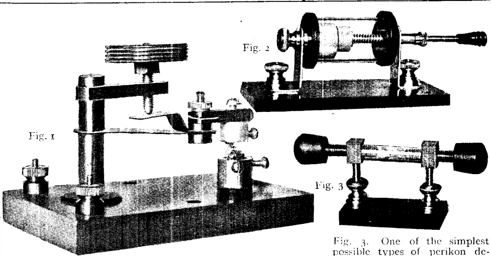
Fig. 1. Chalcopyrites is used as the crystal in the lower cup and zincite in the upper cup. Adjustment is made by the flat spring and knobs. Fig. 2. Perikon detector enclosed in a glass tube to keep the crystals free from dust. The contact is adjustable by a spring and the cups screw over one another
