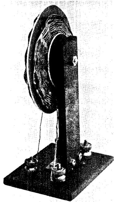
Fig. 5. In this photograph of the completed transformer the method of mounting and connecting the coils is clearly shown
