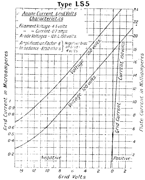
Fig. 17. Characteristics of this loud-speaker valve. Anode voltages should be of the order of 120-150 for the best results, with a generous grid-bias voltage
