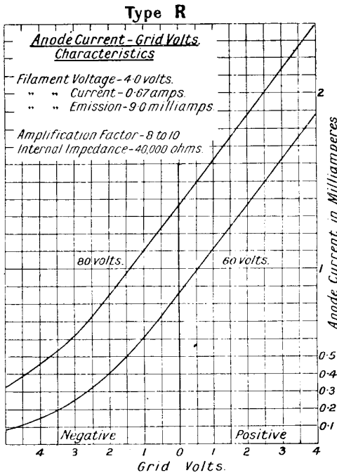
R TYPE MARCONI-OSRAM VALVE
