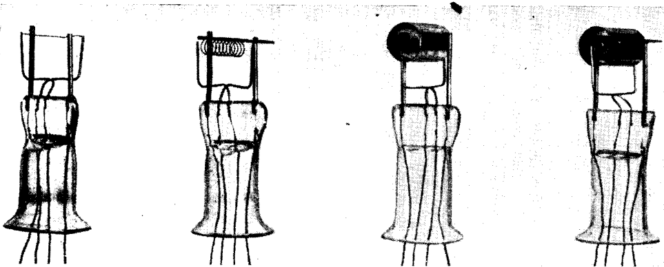
HOW THE MARCONI-OSRAM R VALVE IS ASSEMBLED
