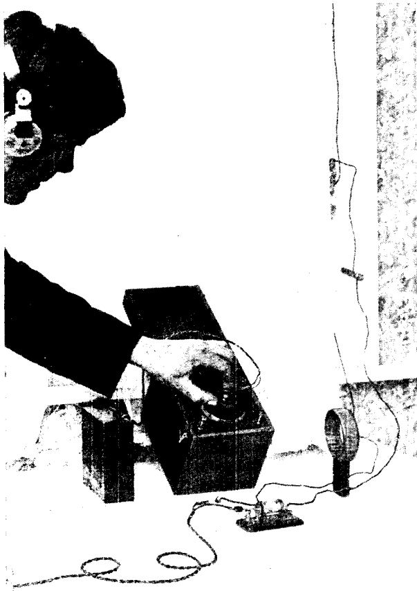
Fig. 4. In this photograph is shown the method of ascertaining the wave-length of an outdoor aerial, using an inductance coil of known wave-length. Note the connexions
