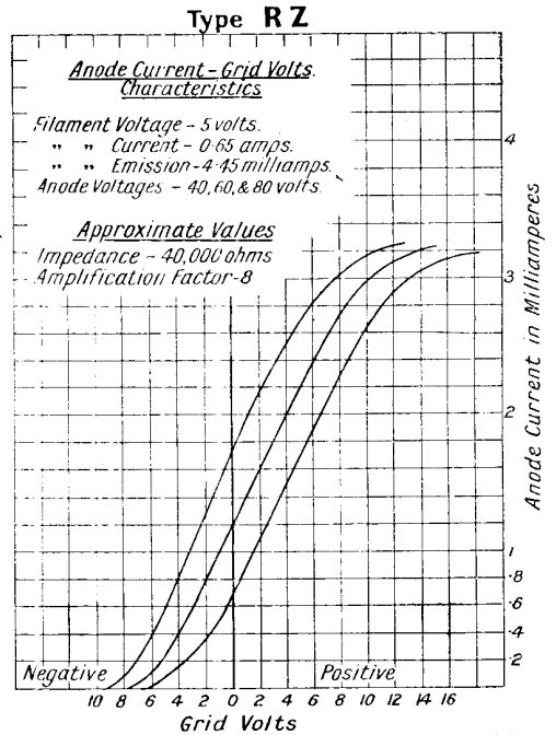
CHARACTERISTICS OF THE RZ VALVE
