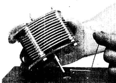
Fig. 6. In wiring the condenser one lead is brought through the panel to the fixed plate beneath the dial
