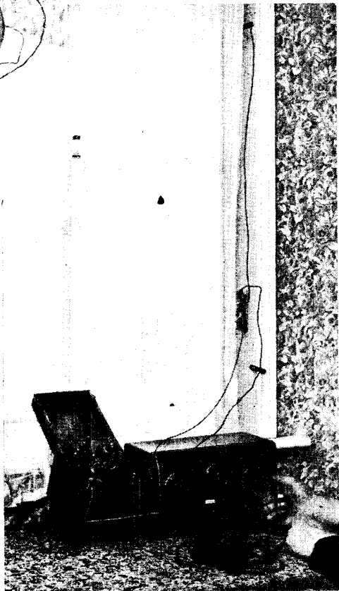
Fig. 5. Where interference from an unwanted transmitter is experienced the wave-meter may often be used as a wave-trap
