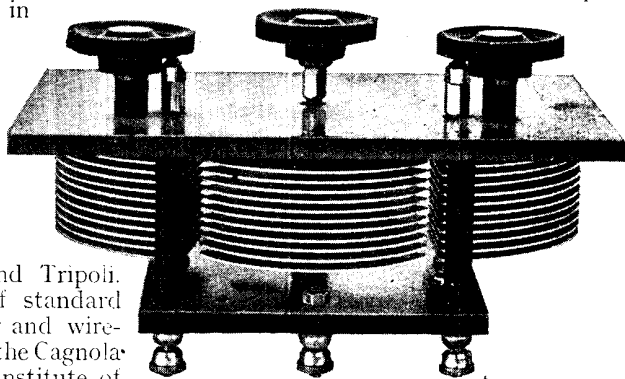
3 E.V.C. TYPE OF CONDENSER
