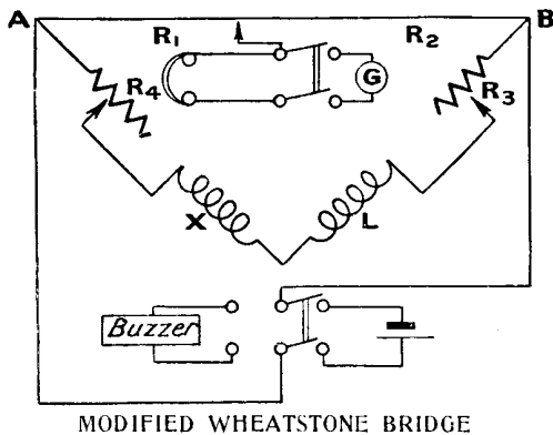
MODIFIED WHEATSTONE BRIDGE
