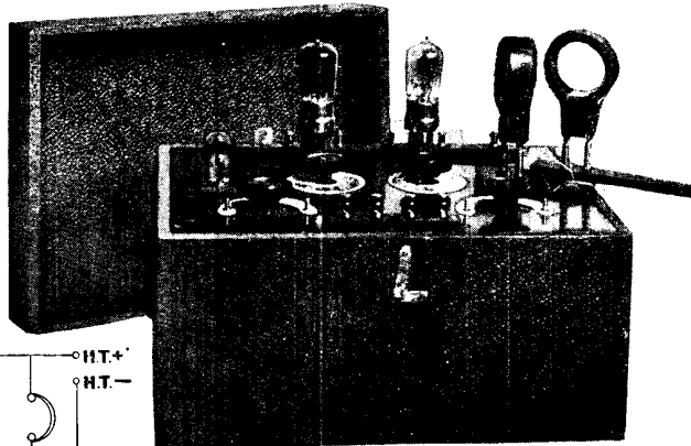
COMPLETE TWO-VALVE AND CRYSTAL SET
