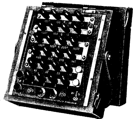
Fig. 5. This is the most common type of Wheatstone bridge. The plugs when taken out increase the total resistance
