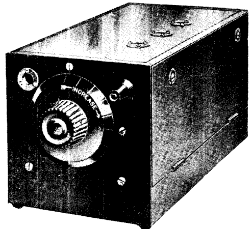
TWO-STAGE AMPLIFIER FOR VALVE SET Fig. 3. Three Weco valves are used in this set, which is a two-stage amplifier
