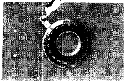
Fig. 4. Plan view of the dial, showing the control knob for the vernier plate of the condenser
