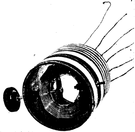
COMMON TYPE OF VARIO-COUPLER
