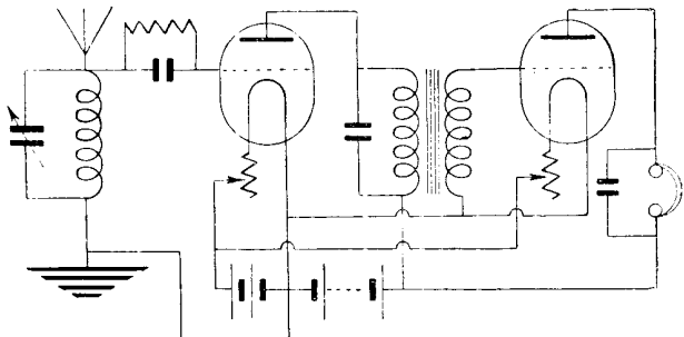
NORMAL TWO-VALVE CIRCUIT
