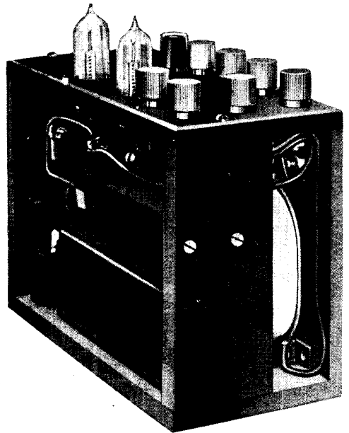
TWO-STAGE L.F. AMPLIFIER FOR CRYSTAL SET Fig. 2. In this amplifier Weco valves are used. The instrument fits the telephone compartment of the Western Electric Co.'s receiver
