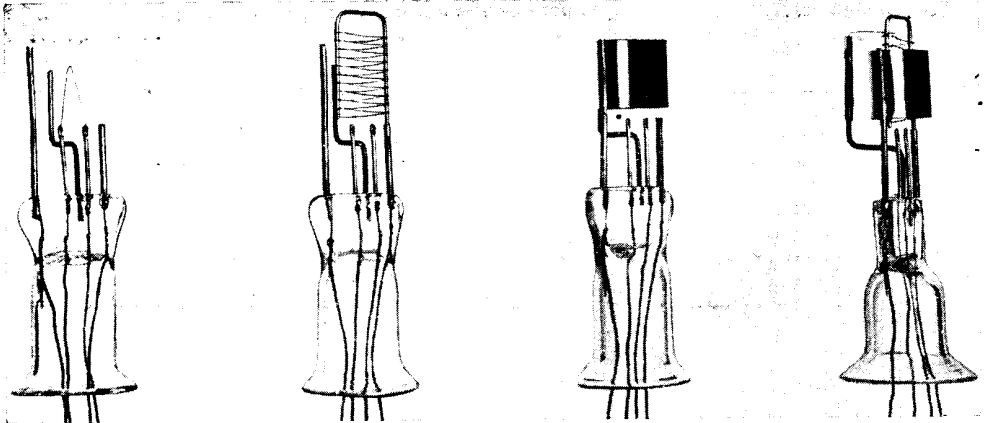
HOW THE MARCONI-OSRAM R5V VALVE IS CONSTRUCTED
