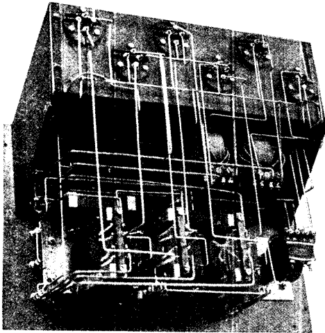
Fig. 12. In this set the various circuits in use are indicated by differently coloured wires
