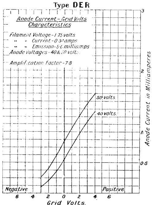
Fig. 18. Curves of the D.E.R type, which requires only a one-cell accumulator and a H.T. battery of 40-50 volts
