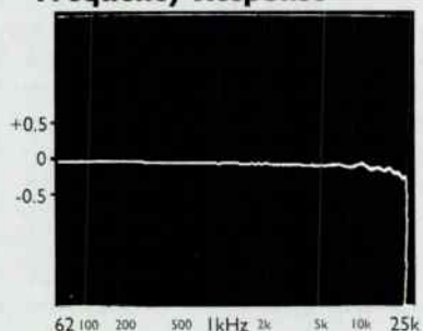
Gently rolled off treble should give a smooth sound
