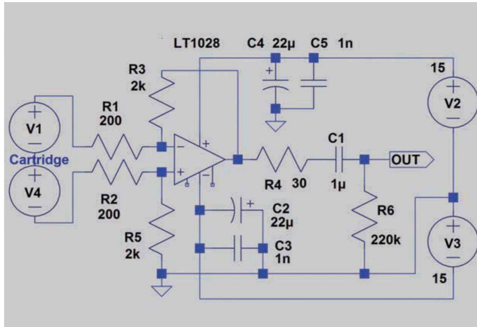
Fig 11 from A Matter of Balance, p89, July 2015 issue. The input impedance is wrong, says Michael Ford.
