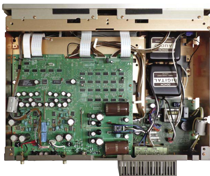
The Panasonic DVD loader and associated circuitry are contained within heavily-screened sections, to avoid contaminating the audio. With the cover removed, all we can see are Denon's audio board and the power supply transformers.
