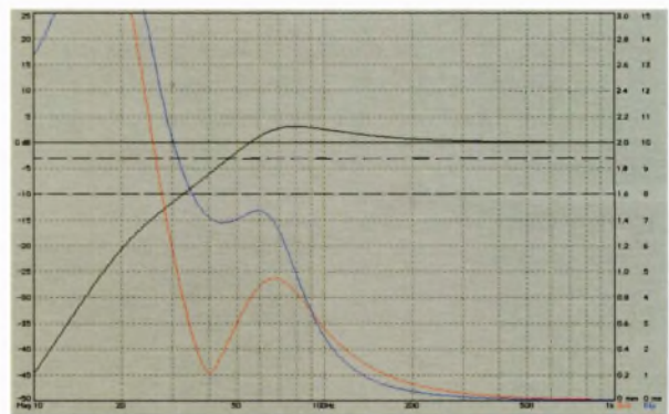
D. Reflex system at elevated voice-coil temperature.
