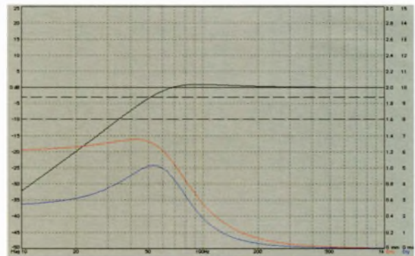
C. Closed box system at elevated voice-coil temperature.
