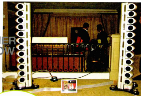
Above: Scaena's 3.4 ribbon/cone line array loudspeaker. Cor!
