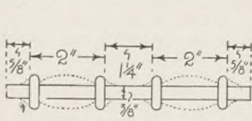
Fig. 3—Shape and size of bails
