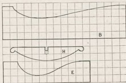
Fig. 2—Outline shape of the various parts
