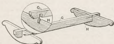
Fig. 5—Details of the rocker portion
