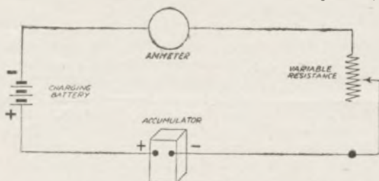
Fig. 2—The circuit diagram
