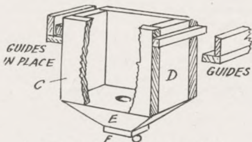
Fig. 1—How the hopper is made and fitted
