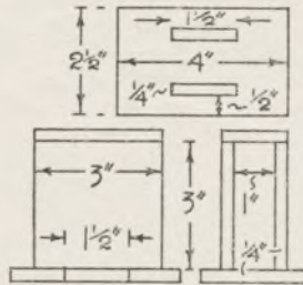
Fig. 3—Sizes of battery box
