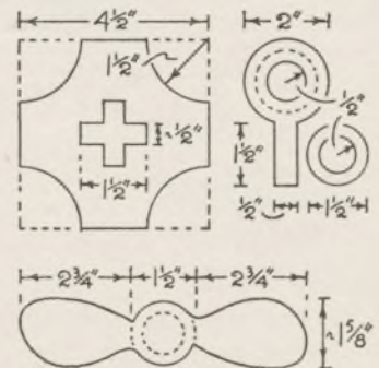
Fig. 2—Dimensions and shapes of base, motor casing and fan blades
